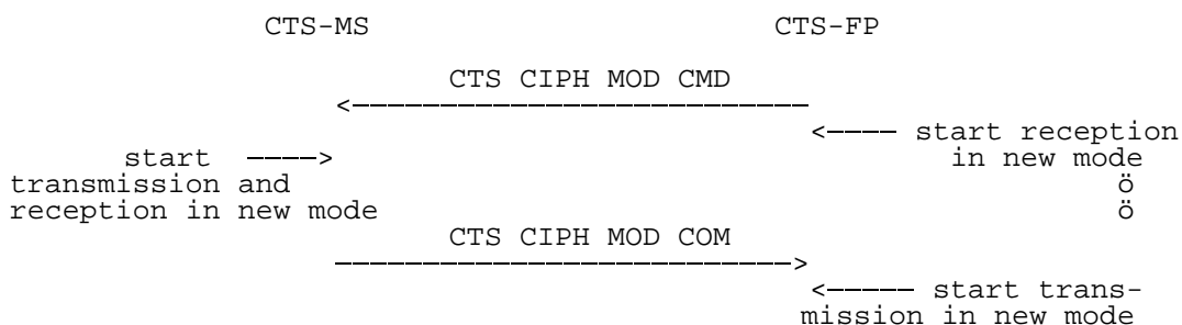
Figure 4.6/GSM 04.56: Ciphering mode setting sequence
