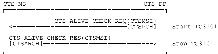
Figure 4.2/GSM 04.56 alive check sequence
