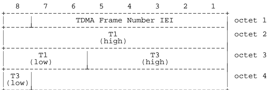
Figure 10.5/GSM 04.56 TDMA Frame Number information element
