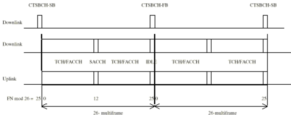
Figure 2: 26-multiframe structure
