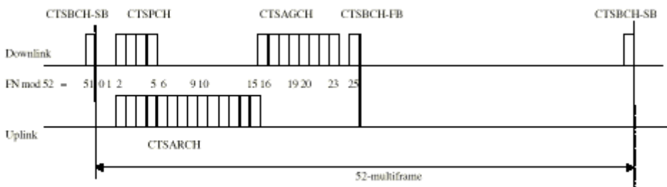
Figure 1: 52-multiframe structure
