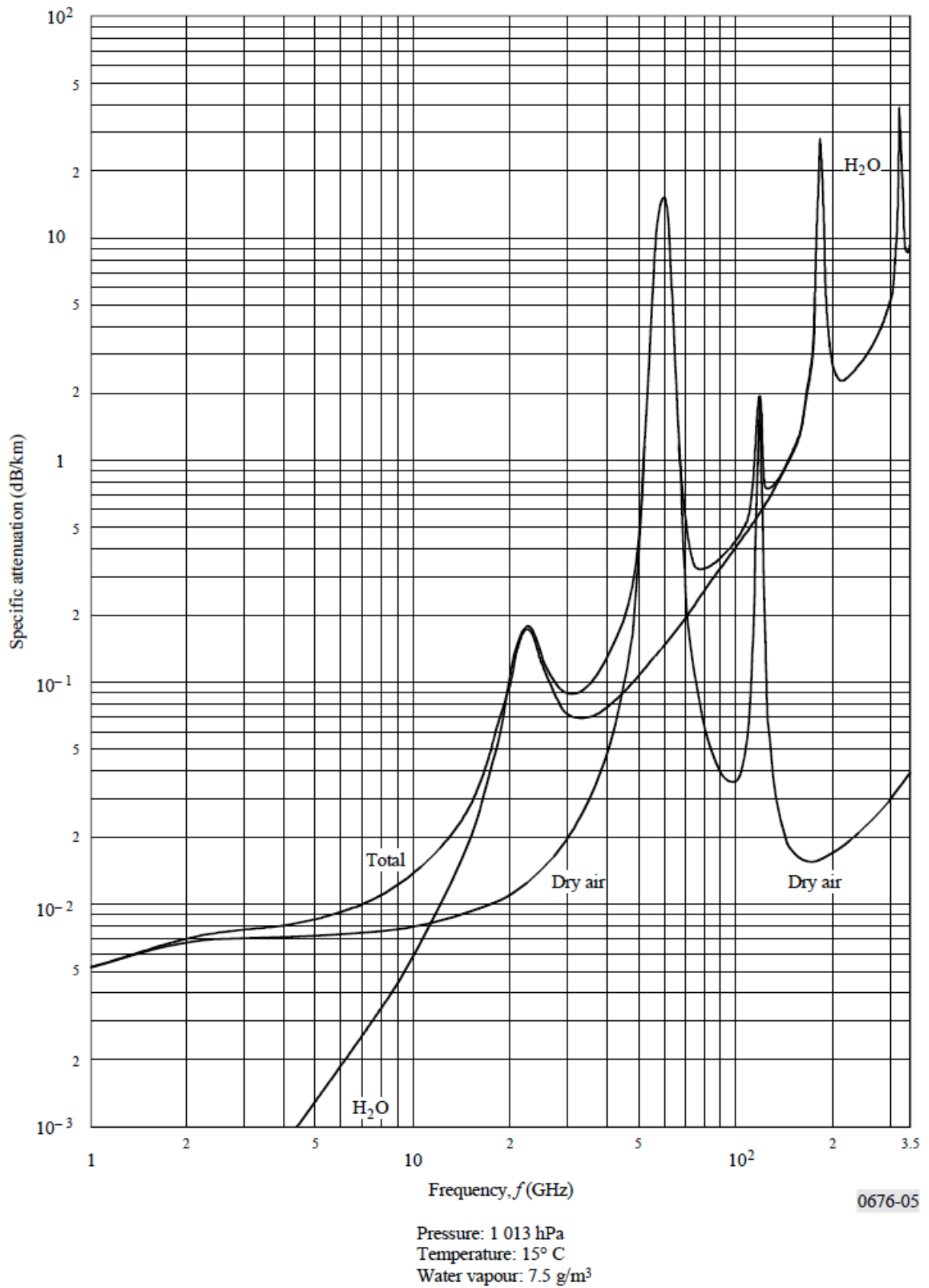
Figure H.1: Specific attenuation due to atmospheric gases in the band 1 GHz to 350 GHz in dB/km
