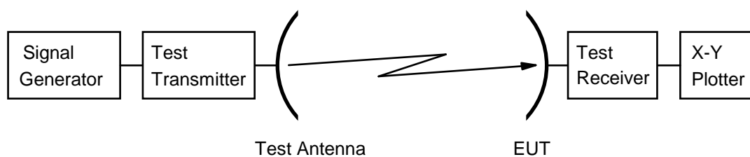
Figure 14: Test arrangement - antenna receive pattern measurement
