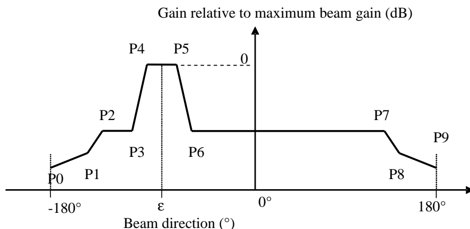
Figure 8: Azimuth RPEs for linear polarized multi-beam sector antennas 3 GHz to 5,9 GHz (defined for each beam)
