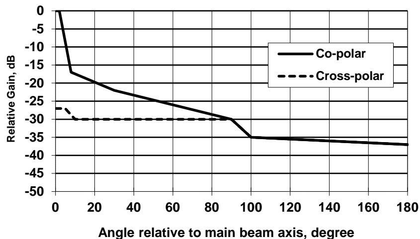
Figure 5: Class DN2 terminal station antenna
