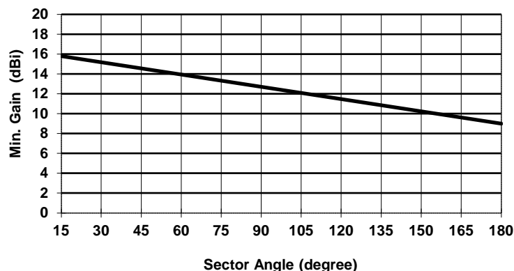
Figure 9: CS Sector Antenna Minimum Declared Nominal Gain Limits
