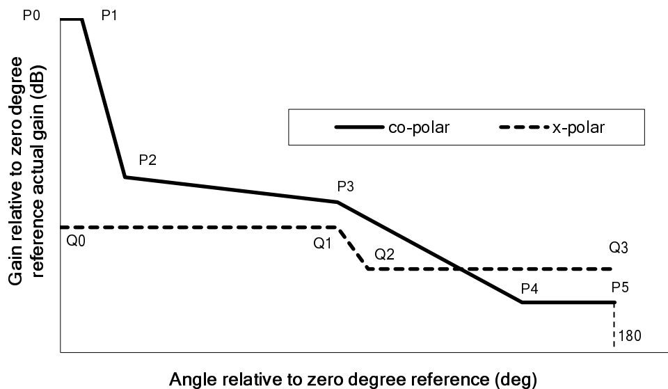
Figure 3: Normalized RPE for DN Azimuth and Elevation
