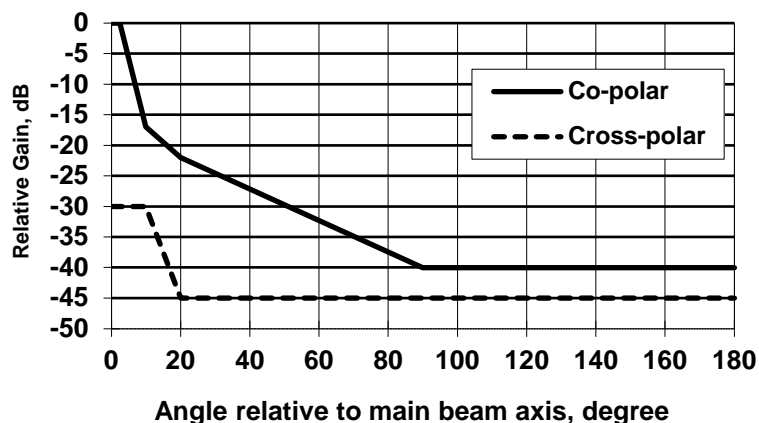
Figure 7: Class DN4 terminal station antenna
