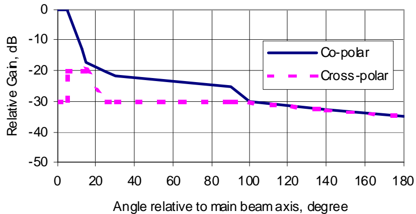
Figure 4: Class DN1 terminal station antenna
