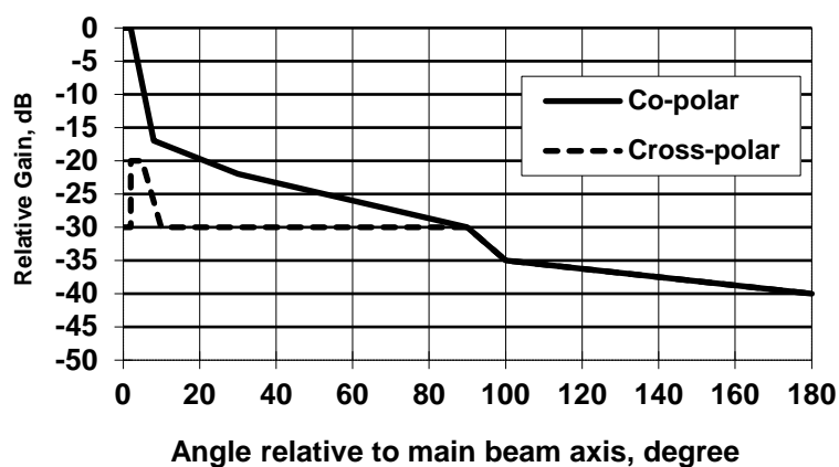
Figure 6: Class DN3 terminal station antenna
