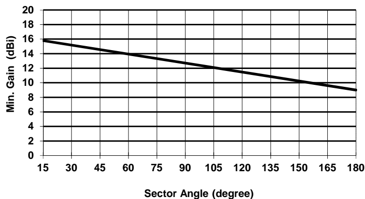
Figure 9: CS Sector Antenna Minimum Declared Nominal Gain Limits
