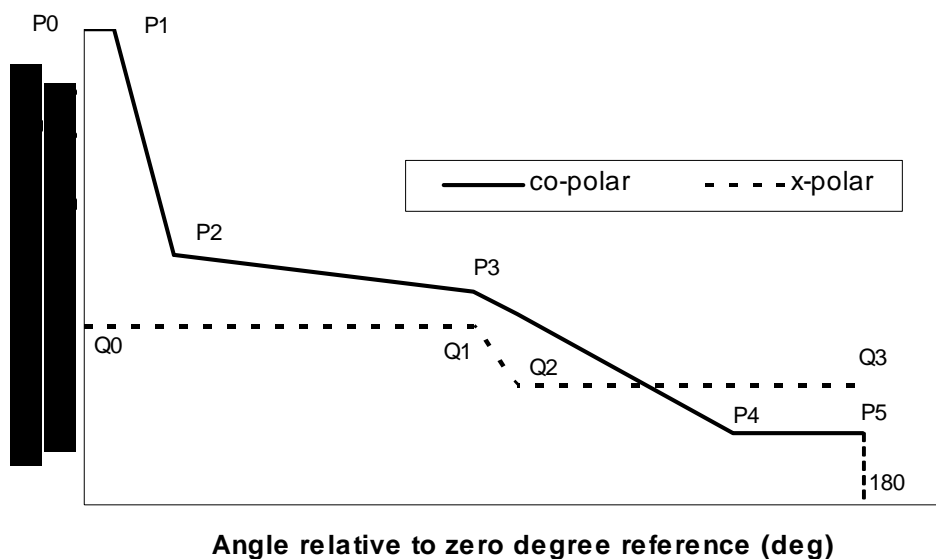
Figure 4: Normalized RPE for DN Azimuth and Elevation
