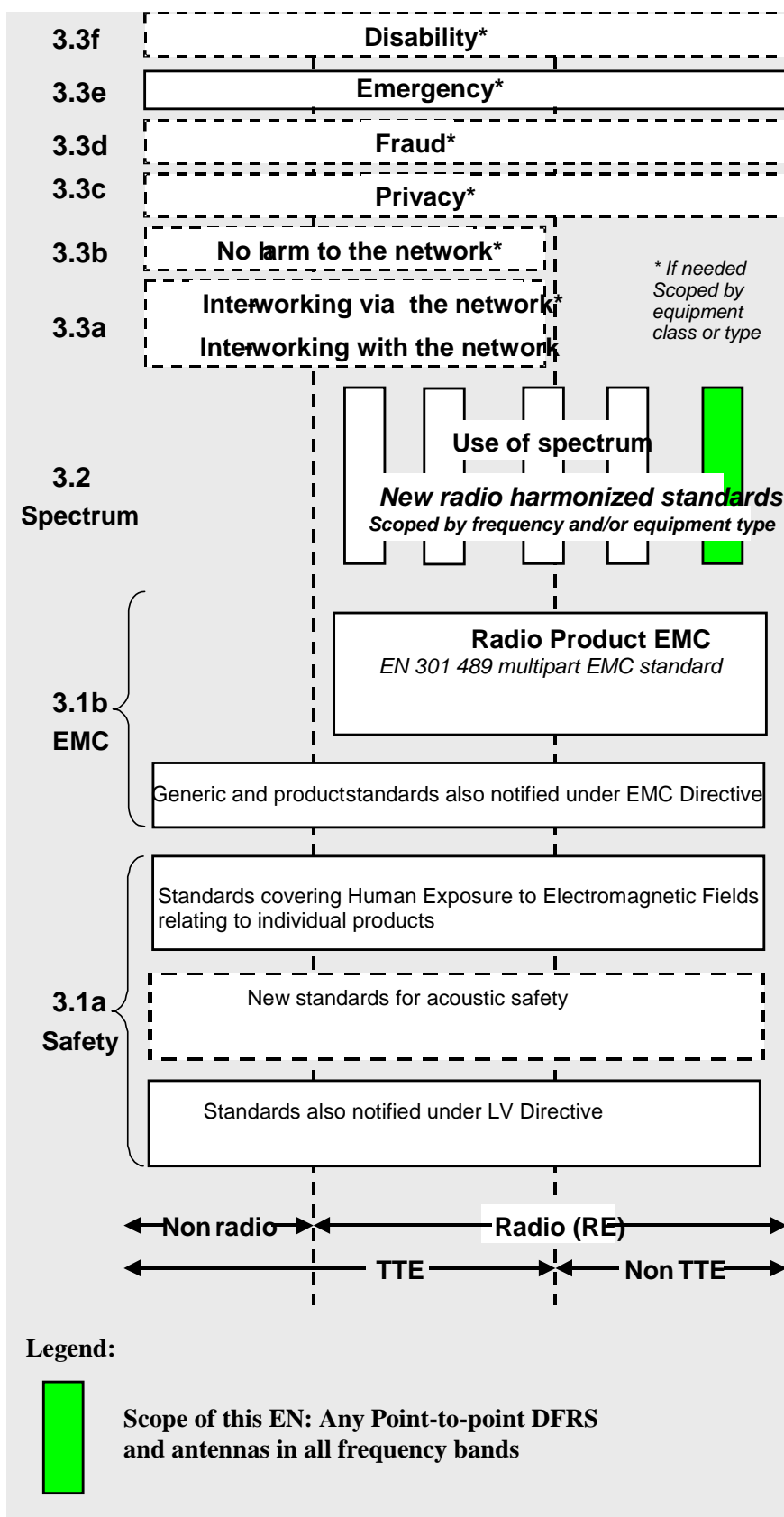
Figure 1: Modular structure for the various standards used under the R&TTE Directive [2]
