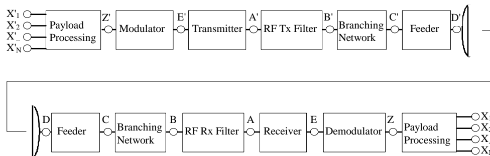
Figure 3: RF system block diagram
