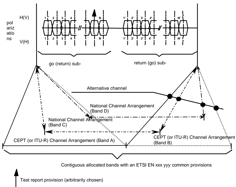
Figure B.1: Test report frequency requirement for equipment intended for single channel operation
