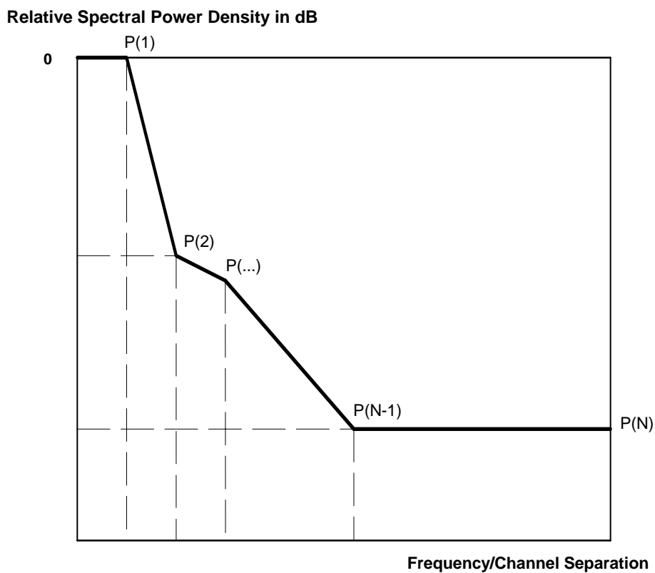
Figure 4: Power spectrum mask - Generalized Form
