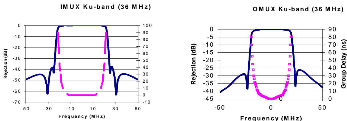
Figure H.13: IMUX and OMUX characteristics
