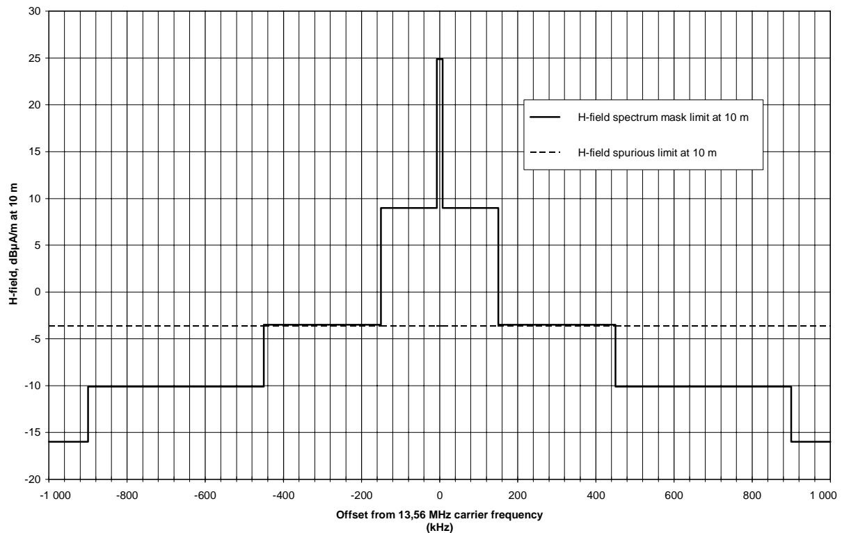
Figure 1: Transmitter spectrum mask
