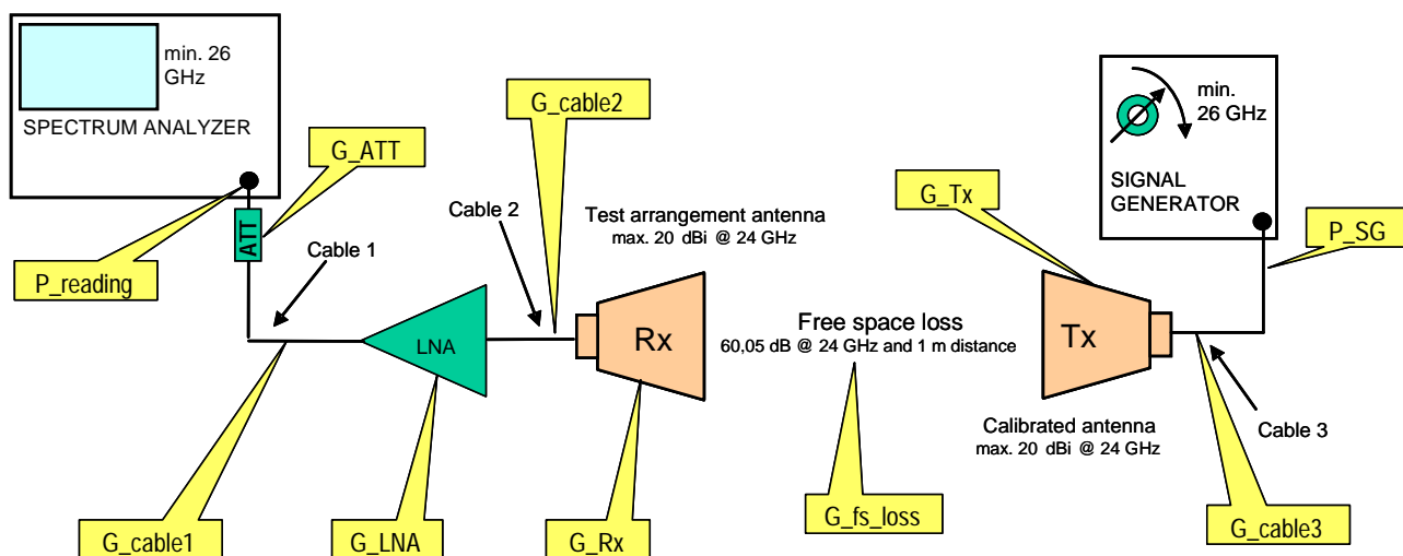
Figure 1: Calibration set-up configuration (example for 1m Rx to Tx free space distance)
