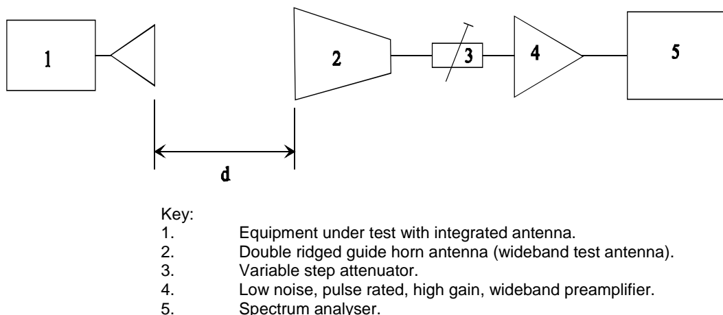
Figure 4: Test set-up for power density measurements of transmitters operating in the 22,000 GHz to 26,625 GHz band
