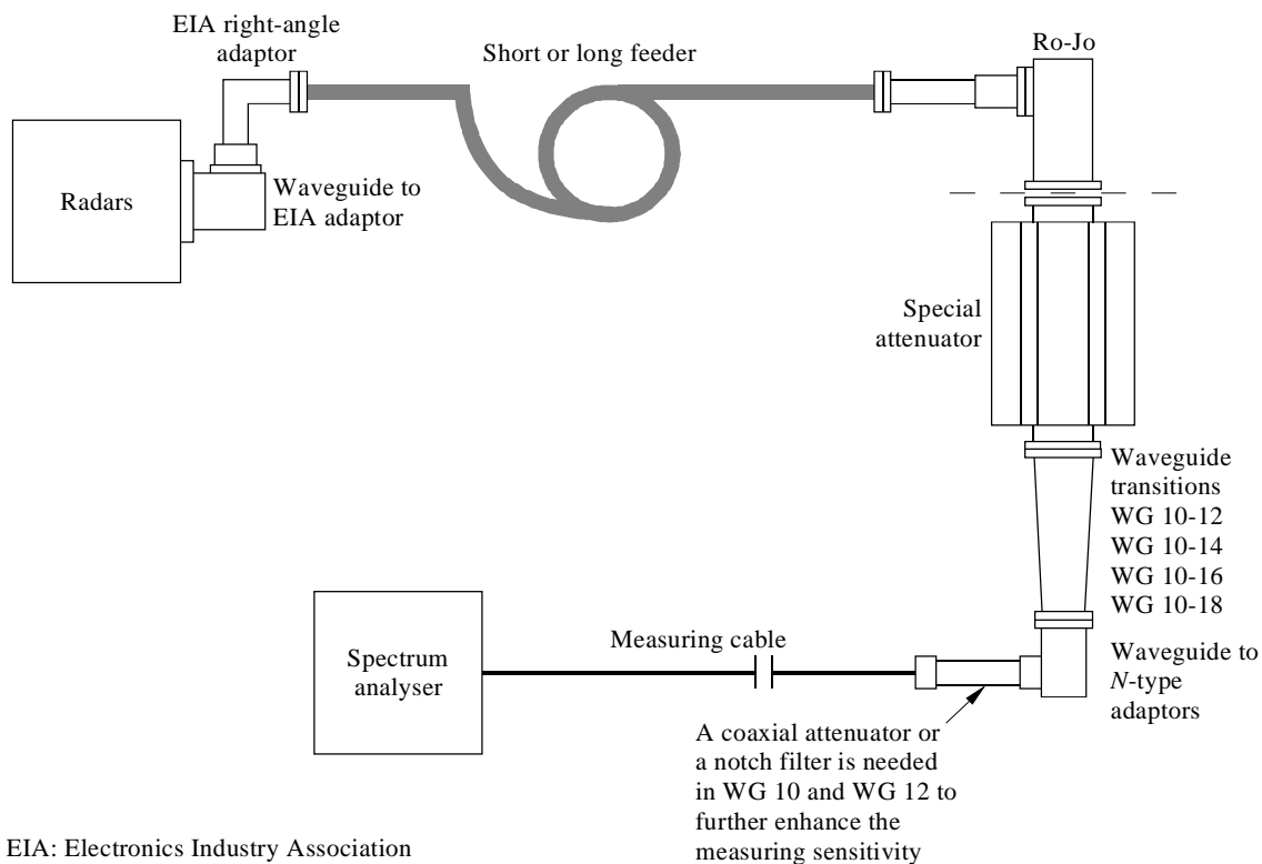
Figure B.1: Measurement at the Ro-Jo port
