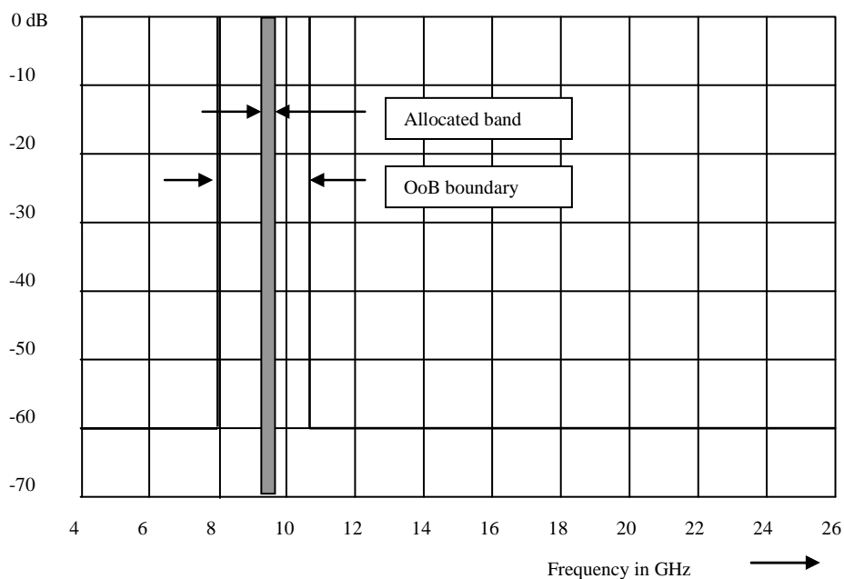
Figure B.3: Maximum permitted spurious emissions power level
