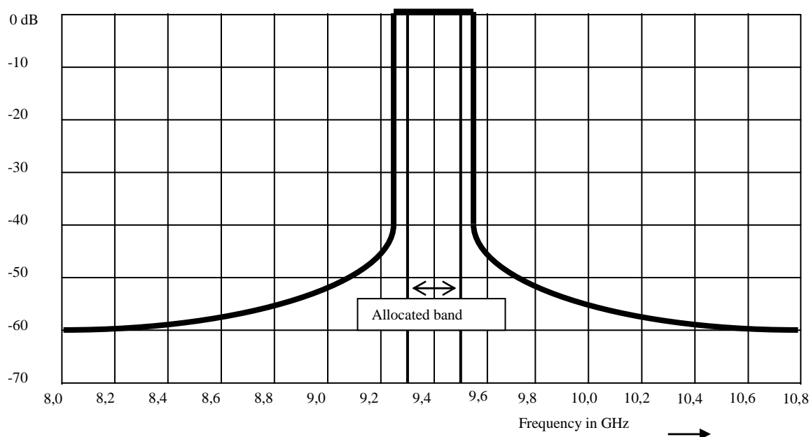
Figure B.2: Maximum permitted Out Of Band-emissions power level
