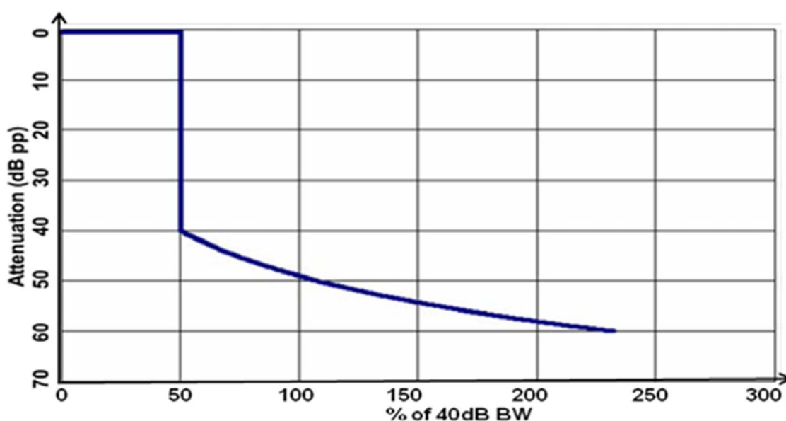
Figure 1: OoB mask for all non-excluded radar waveforms in clause 7.4.3.2
