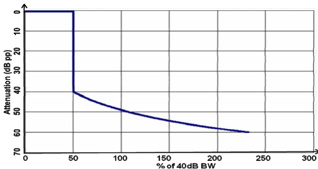
Figure 1: OoB mask for all non-excluded radar waveforms in clause 4.2.4.1.5
