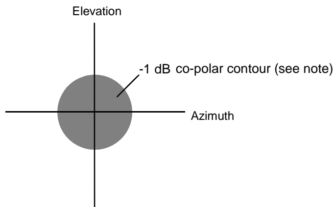
Figure 31: Category 2 mask for XPD measurements around the main beam axis
