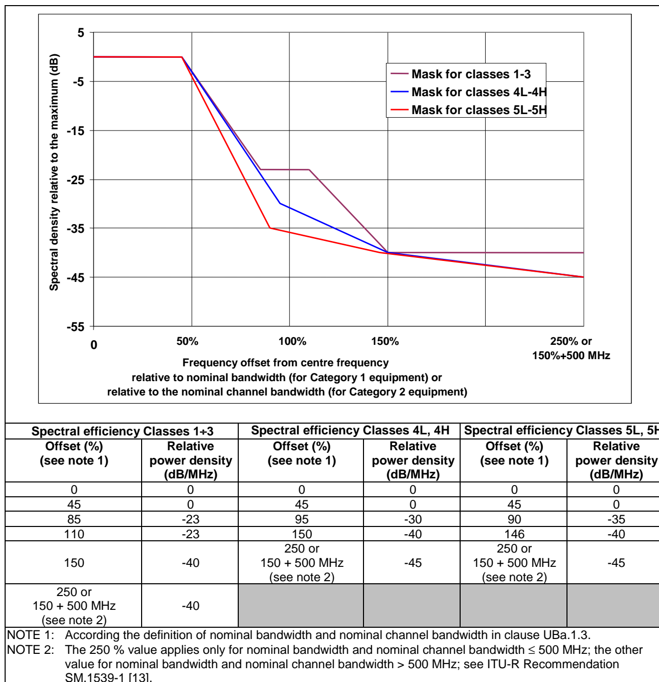
Figure UBa.3: TX EIRP (or Pout) spectral density mask
