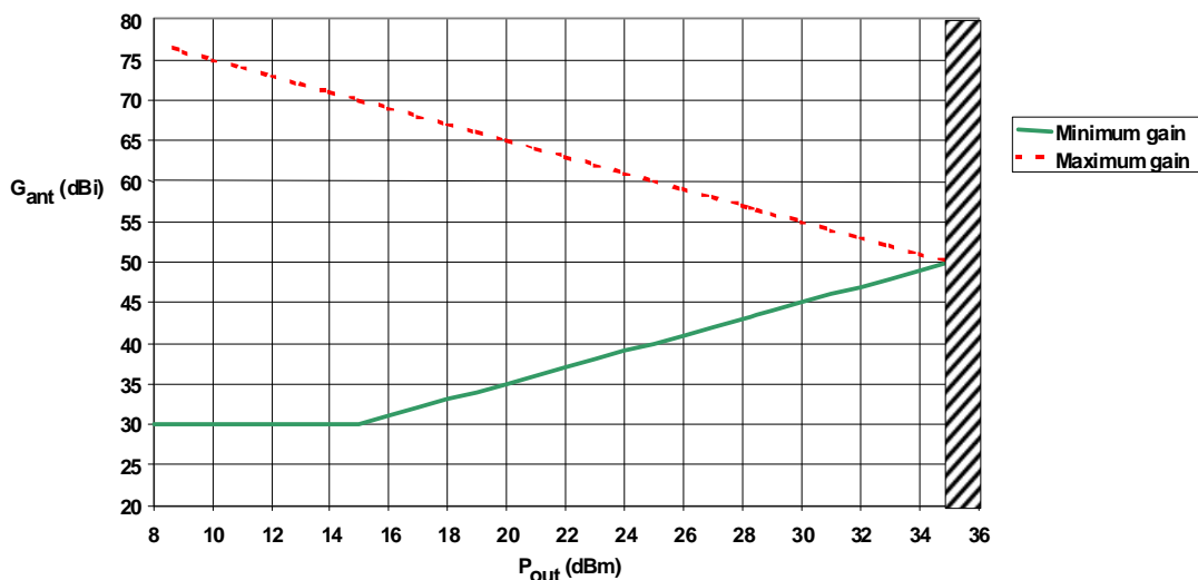
Figure UB.1: Graphical relationship among EIRP limitation, antenna gain and output power
