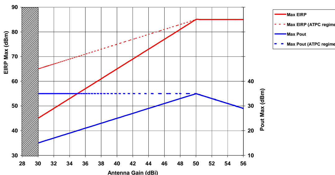
Figure UB.1: Graphical relationship among EIRP limitation, antenna gain and output power
