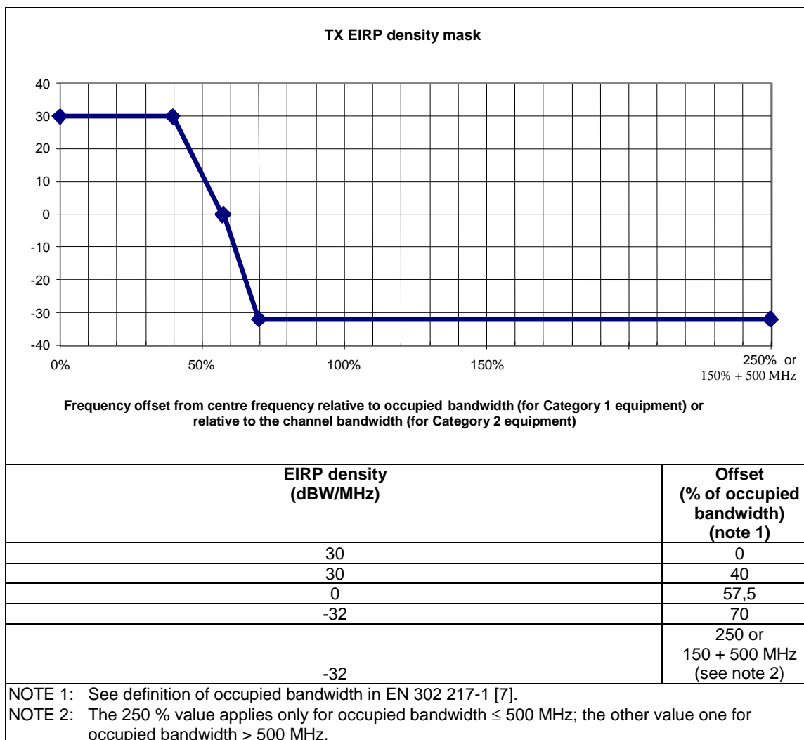
Figure UB.3: Tx EIRP spectral density mask
