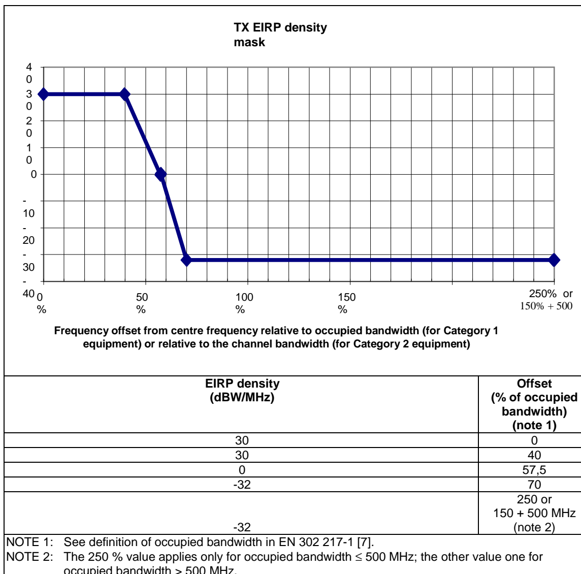
Figure UB.3: Tx EIRP spectral density mask
