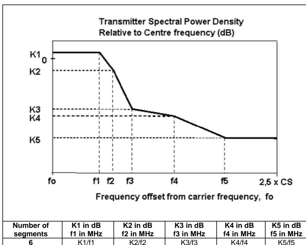
Figure 5: Six segment spectrum mask
