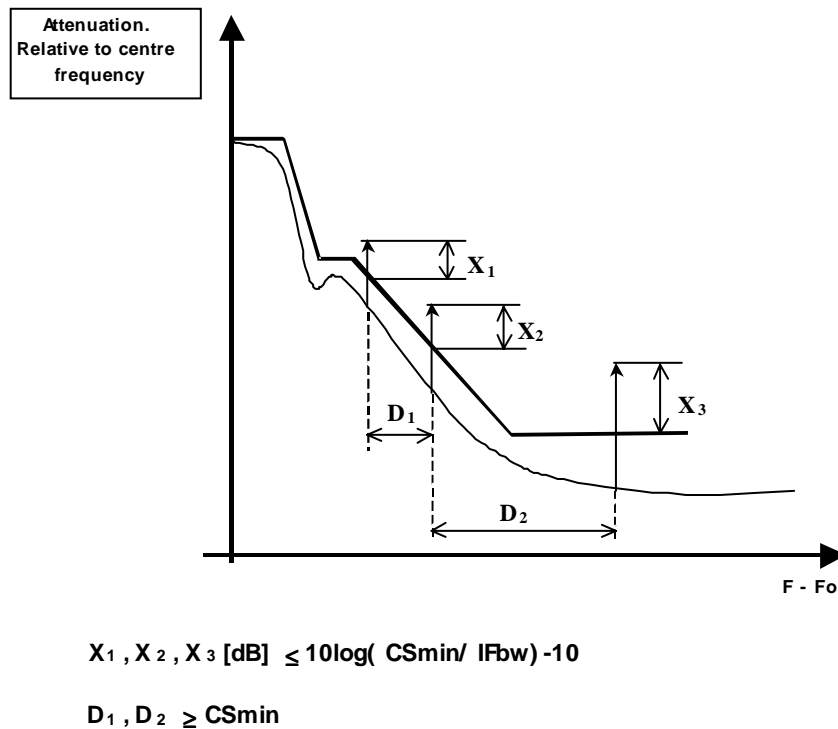
Figure 7: CW lines exceeding the spectrum mask (typical example)
