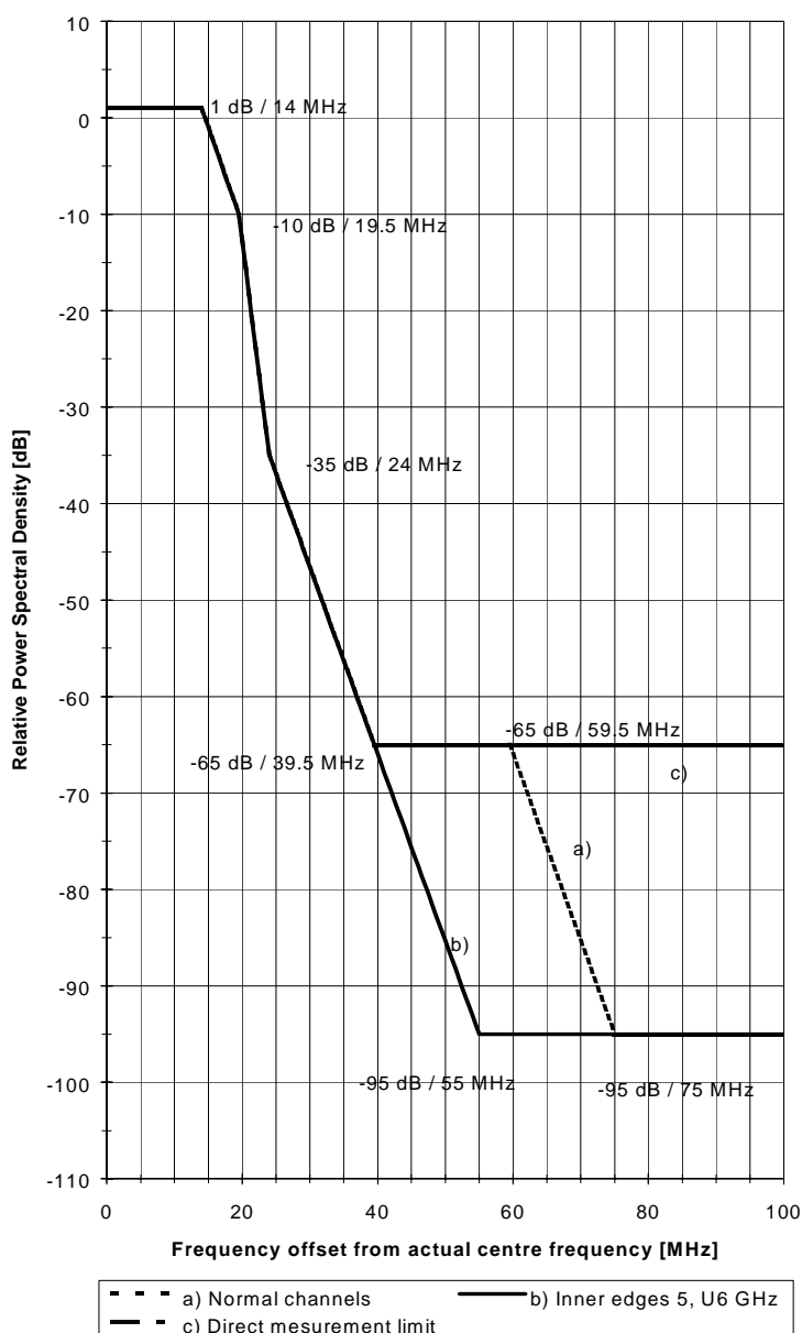
Figure C.1: Limits of power spectral density (reference point B')
