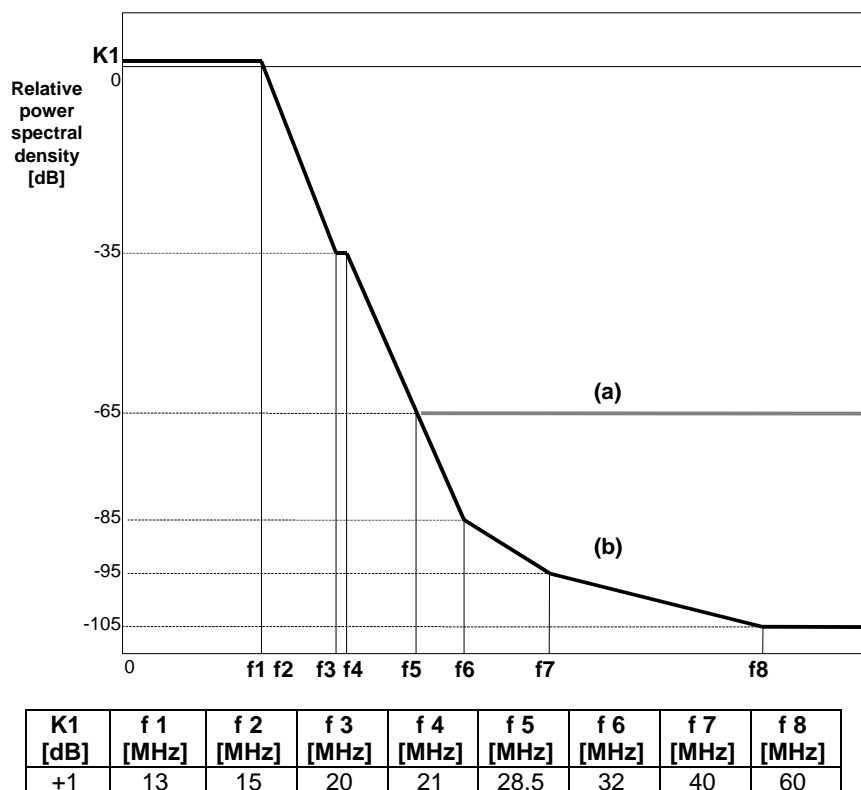
Figure B.2: Limits of Power Spectral Density for the innermost channels (class 5 A), L6 GHz band (reference point B')
