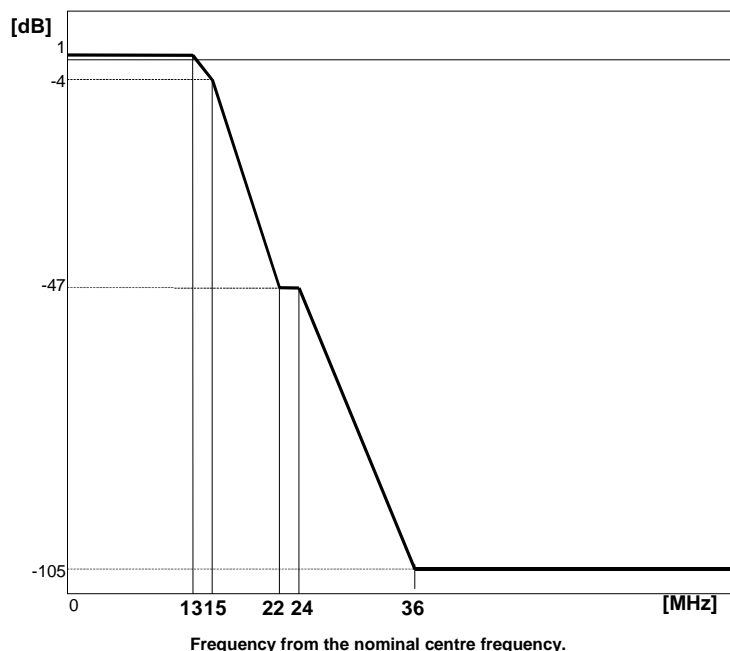
Figure B.4: Overall minimum receiver selectivity of the inner side of innermost receiver for L6 GHz band (class 5 A)
