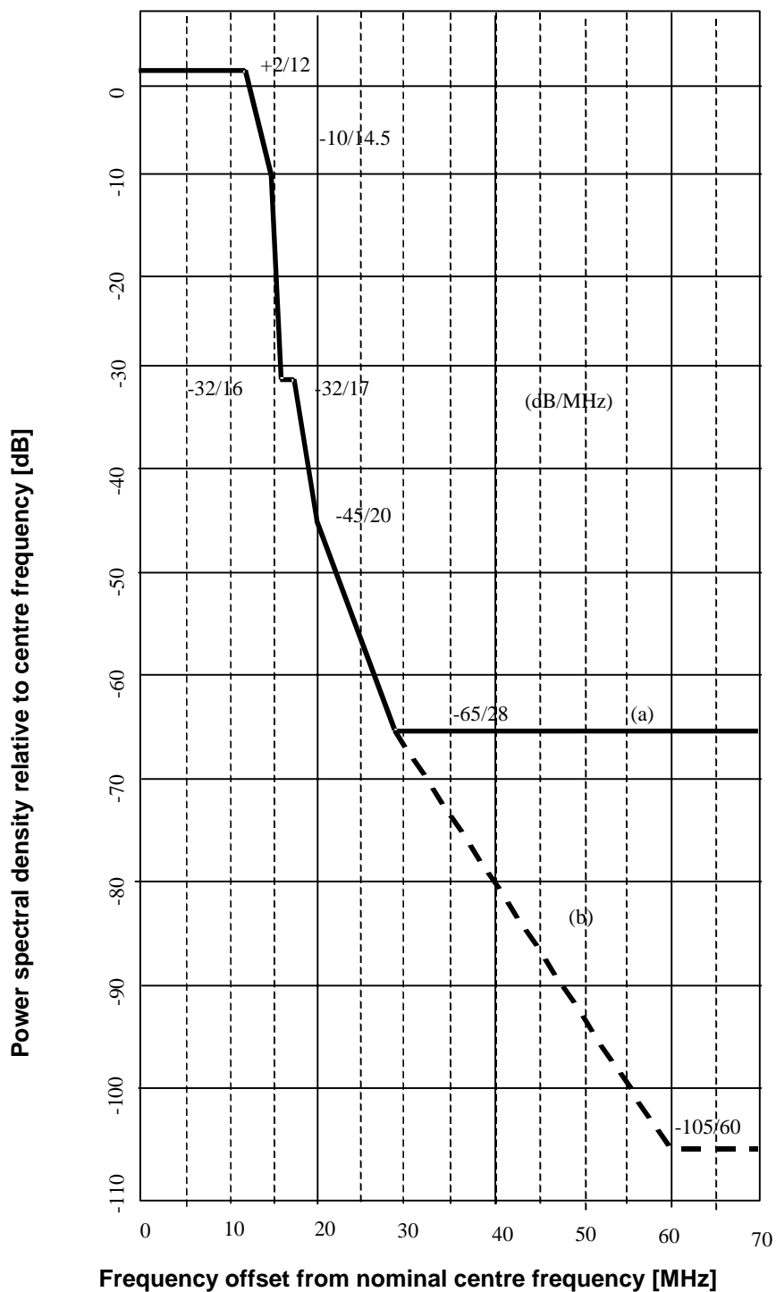
Figure B.6: Spectrum mask for frequency bands with 28 MHz channel separation: (a) limit for direct measurement (b) normal channels (valid also for the innermost channels with 56 MHz centre gap)
