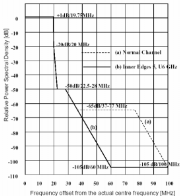
Figure C.4: Limits for multi-carrier systems
