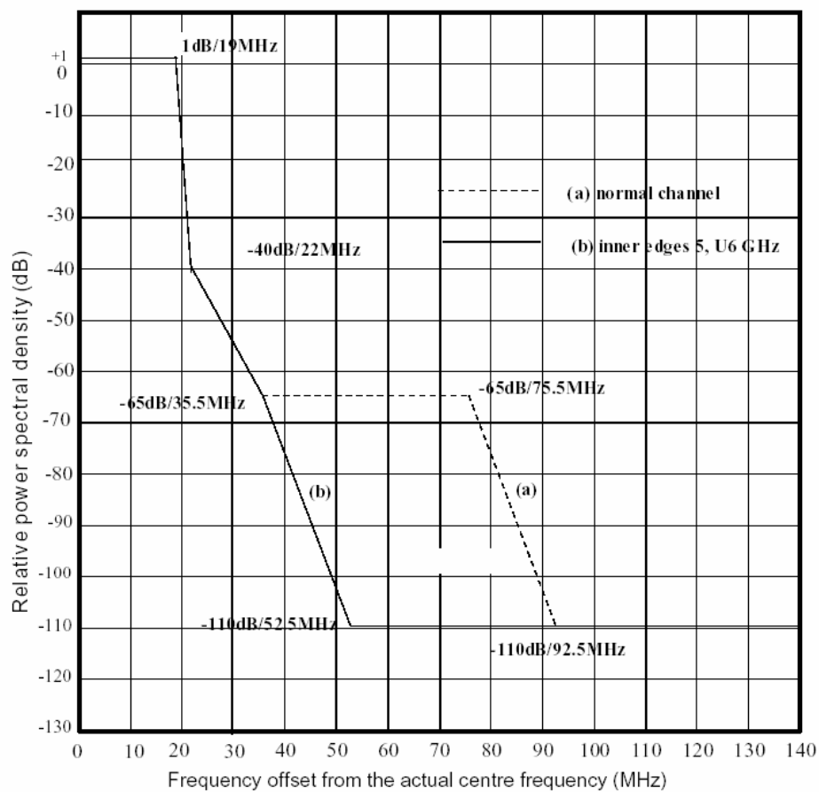
Figure C.3: Limits for single carrier systems
