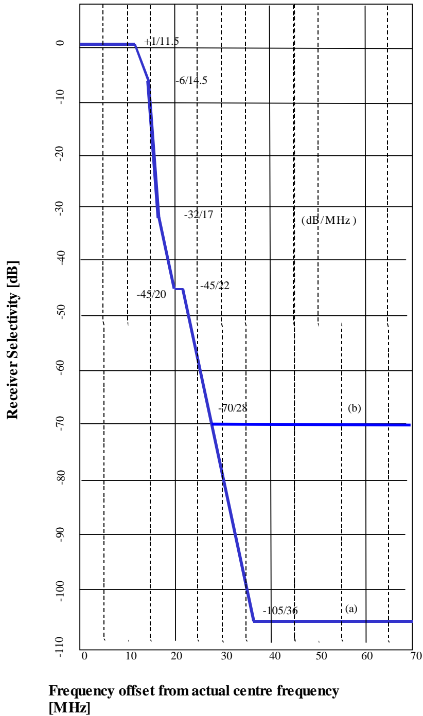
Figure B.7: Limits for the receiver selectivity for the inner edges of the innermost channels in the 6L GHz band (a) Systems sharing the same branching) (b) Systems sharing the same site on different antennas
