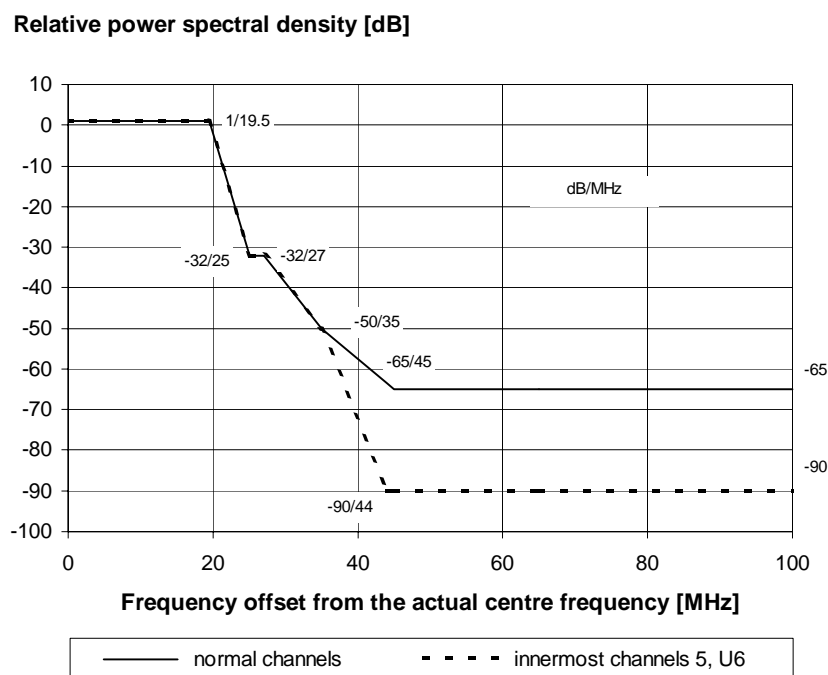
Figure C.2: Limits of spectral power density
