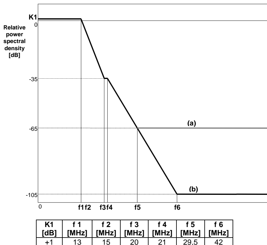
Figure B.3: Limits of Power Spectral Density for the inner edges of innermost channels (class 5 A) in the 7 GHz band with 56 MHz co-polar centre gap (reference point B')
