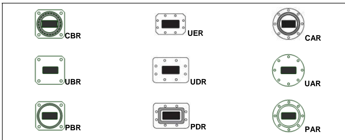
Figure 2: Waveguide Flange Shapes
