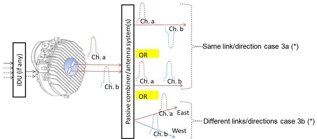
Figure C.3: Example of Channels aggregation/dual-port equipment
