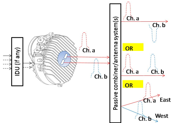
Figure C.3: Example of Channels aggregation/dual-port equipment
