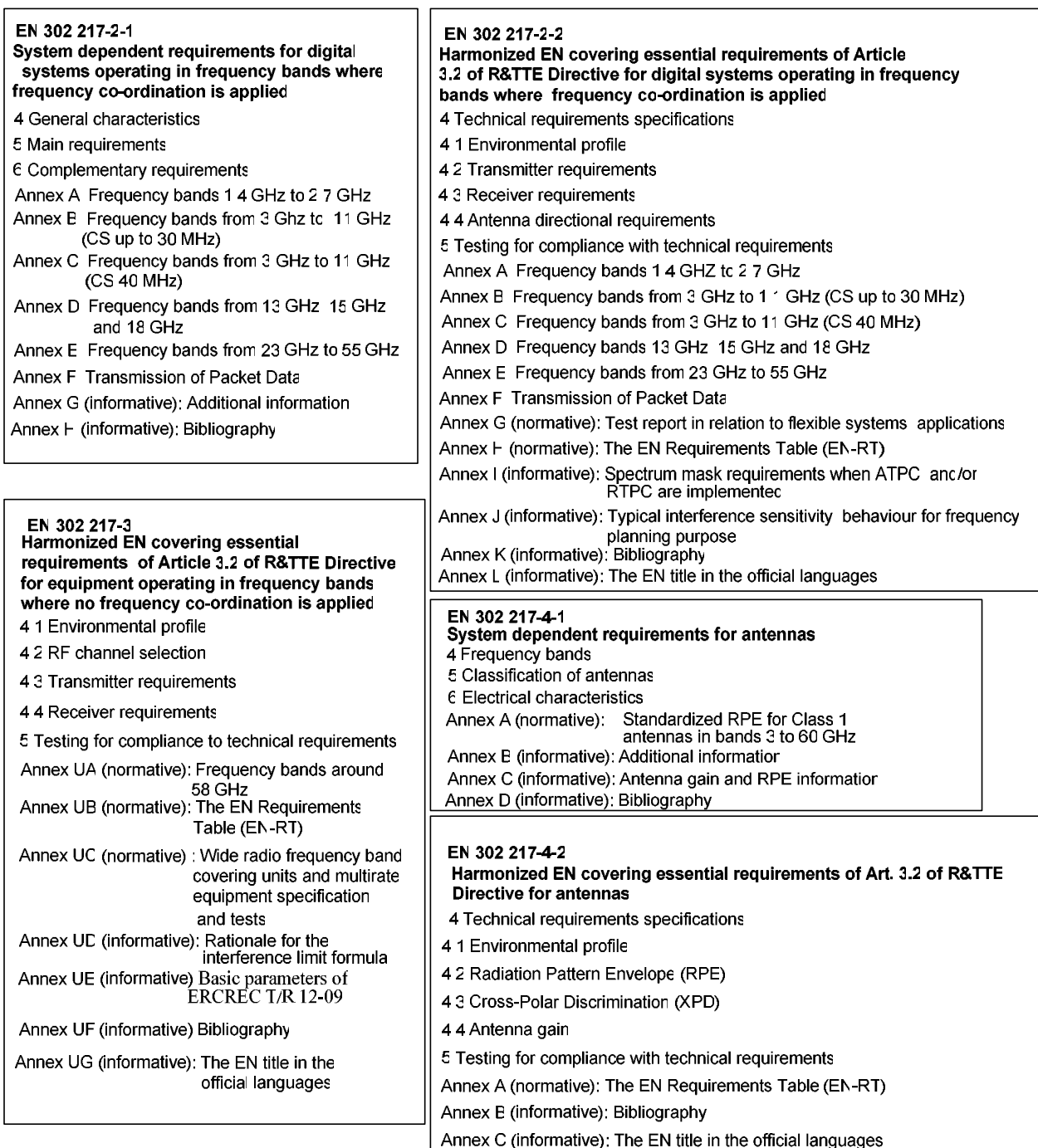
Figure 0: Structure of this EN 302 217 series
