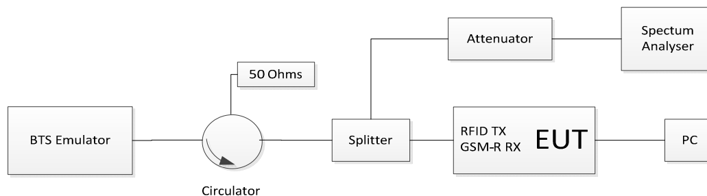
Figure 10a: Set-up of equipment for mitigation test using splitter
