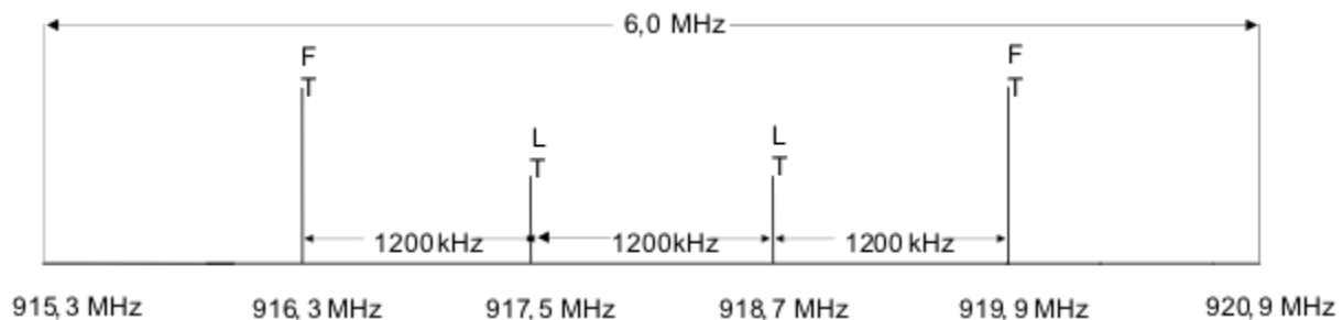
Figure 4: Tests on a single sample for equipment in the upper band
