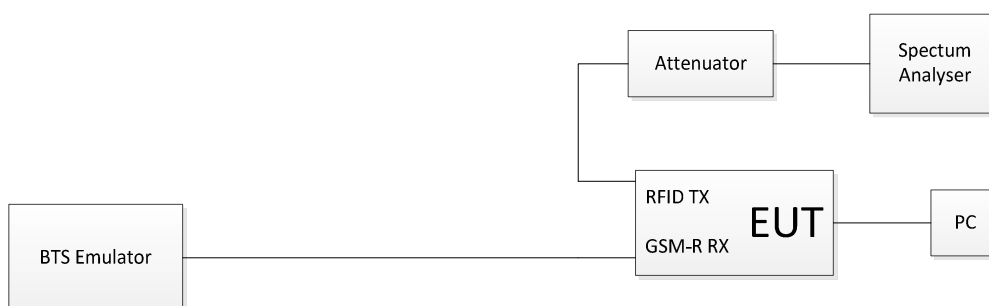
Figure 10b: Set-up of equipment for mitigation test
