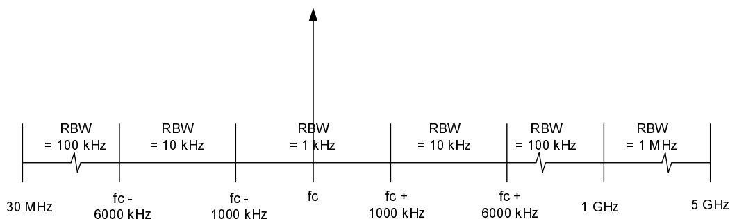
Figure 13: Resolution bandwidths for tag emissions in the upper band
