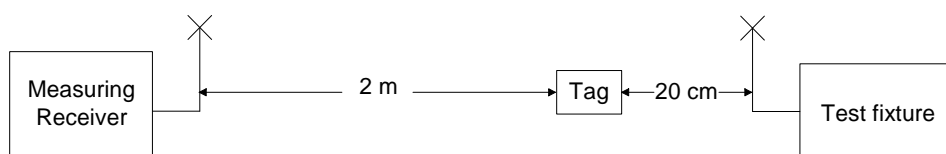
Figure 5: Measurement of tag emissions
