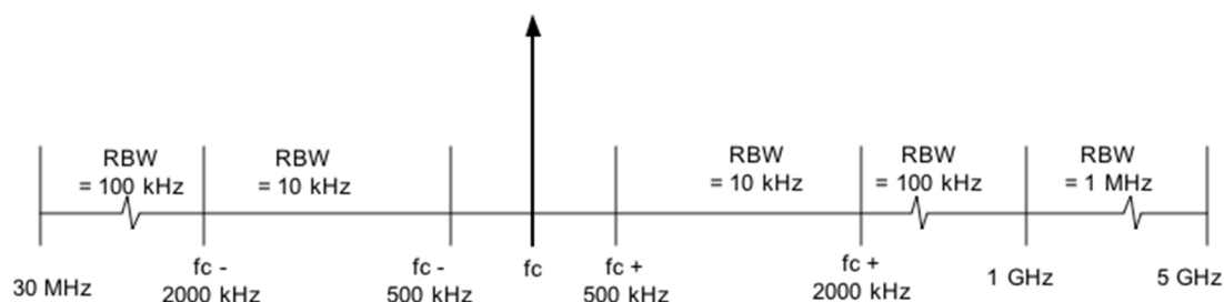
Figure 8: Resolution bandwidths for spurious emission in the lower band
