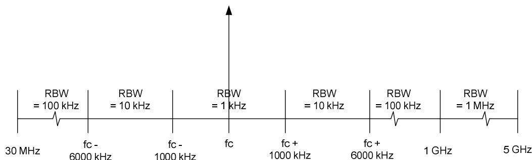
Figure 18: Resolution bandwidths for tag emissions in the lower band
