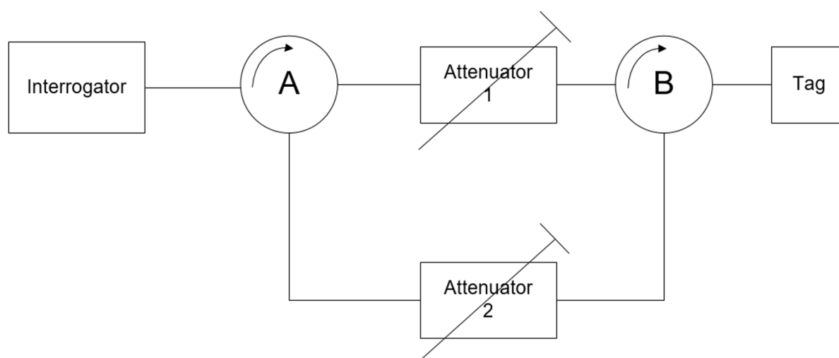
Figure 12: Conducted test set up for receiver sensitivity
