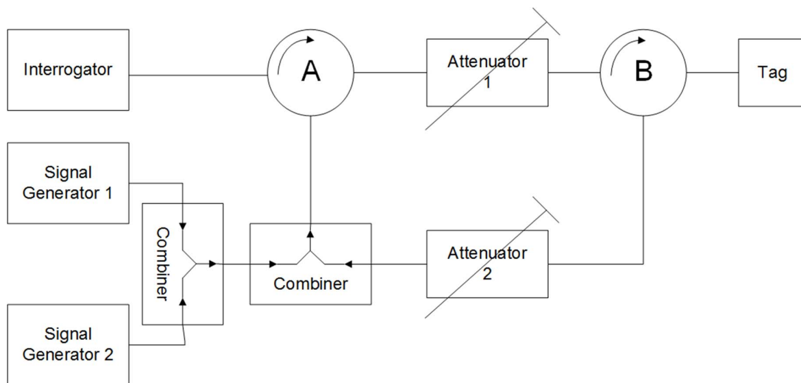
Figure 15: Conducted test set up for intermodulation response rejection
