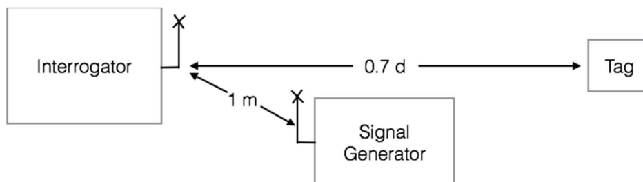
Figure 10: Radiated test set up for adjacent channel selectivity
