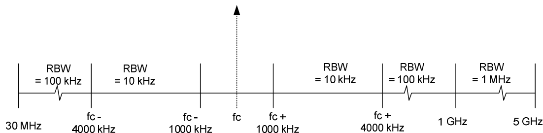
Figure 9: Resolution bandwidths for spurious emission in the upper band
