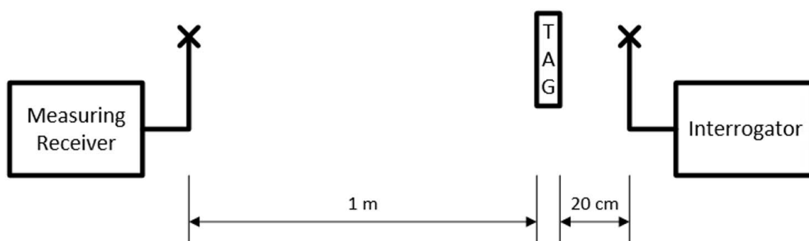
Figure 16: Measurement of tag emissions
