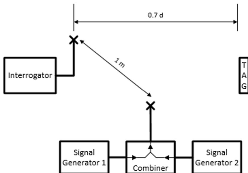
Figure 14: Radiated test set up for intermodulation response rejection
