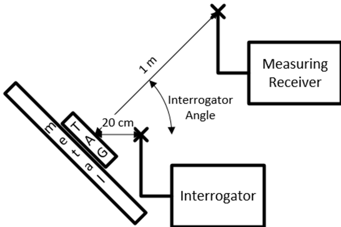
Figure 17: Measurement of tag emissions with metal
