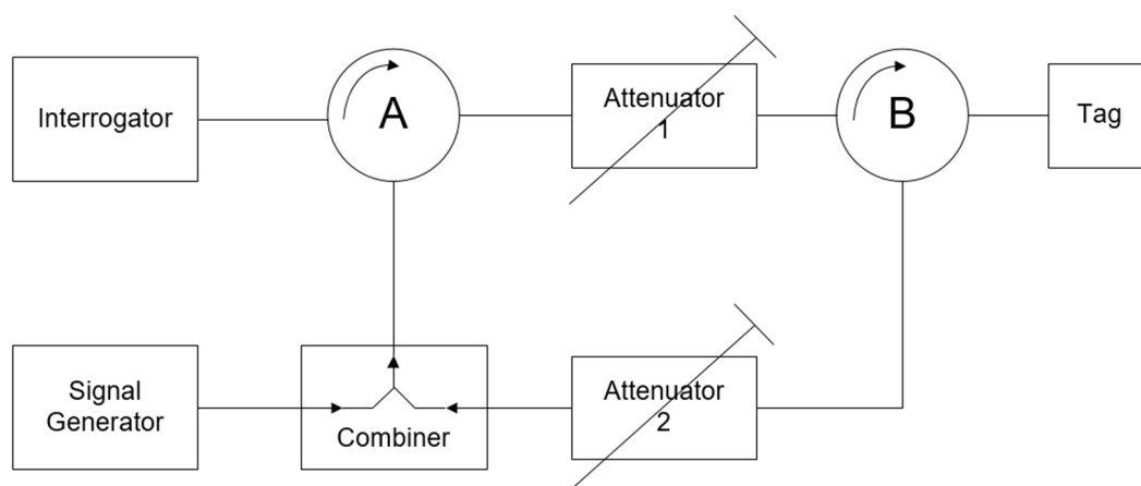
Figure 11: Conducted test set up for adjacent channel selectivity
