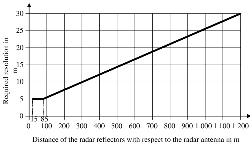
Figure B.4: Required Azimuthal Resolution depending on the range
