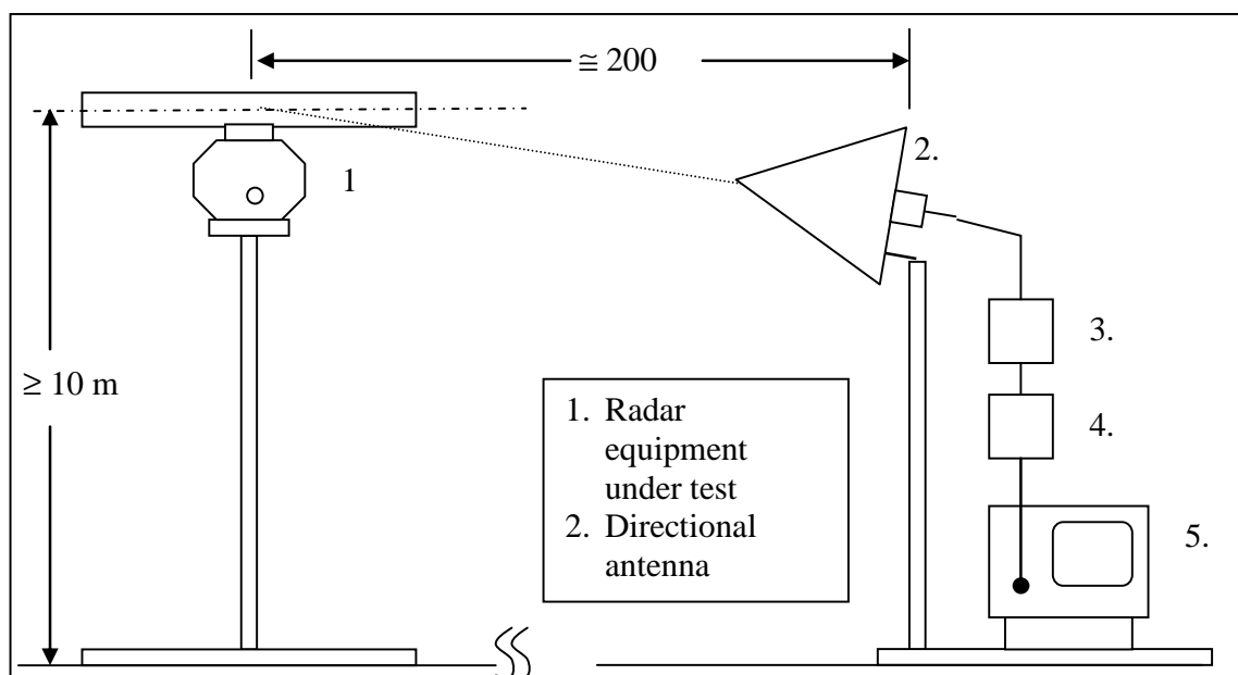
Figure C.2: Measurement of spurious emissions and out of band emissions, placement of components
