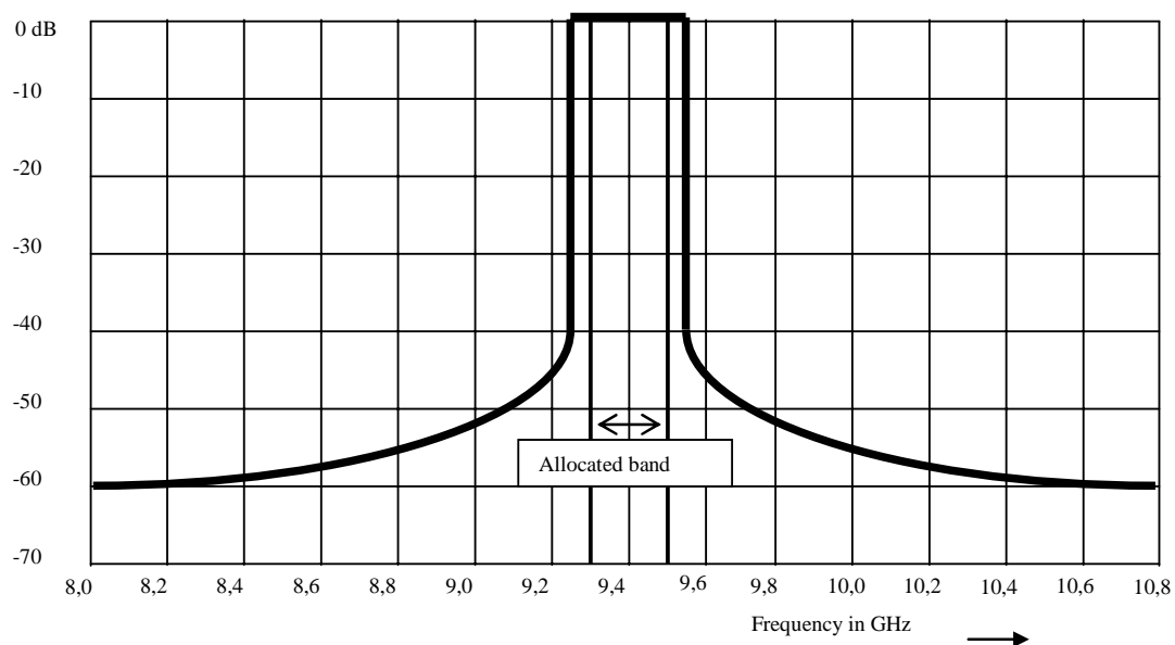
Figure C.3: Maximum permitted out-of-band-emissions power level
