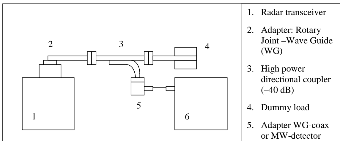
Figure C.1: Measurement of the operation frequency and the pulse power
