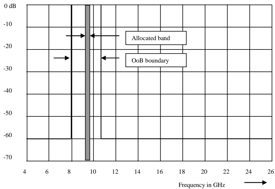
Figure C.4: Maximum permitted spurious emissions power level
