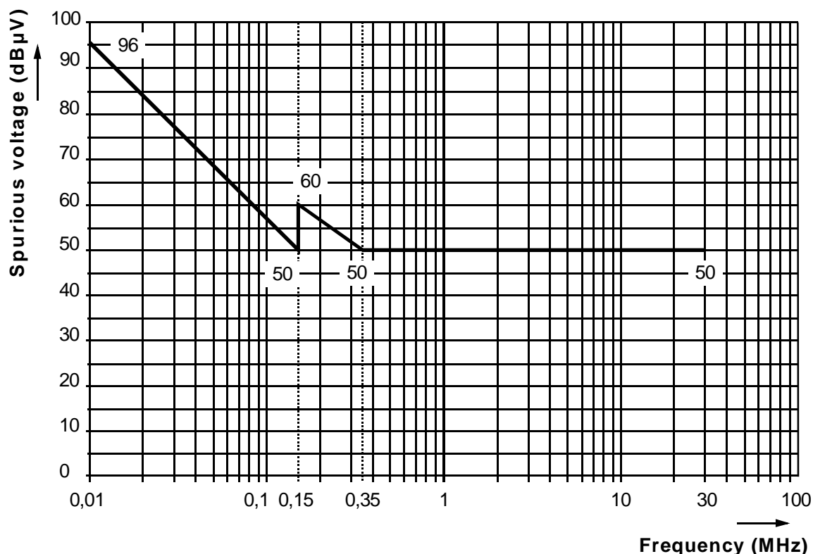
Figure 1: Conducted emissions
