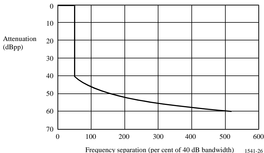
Figure 2: Oob mask for primary radars
