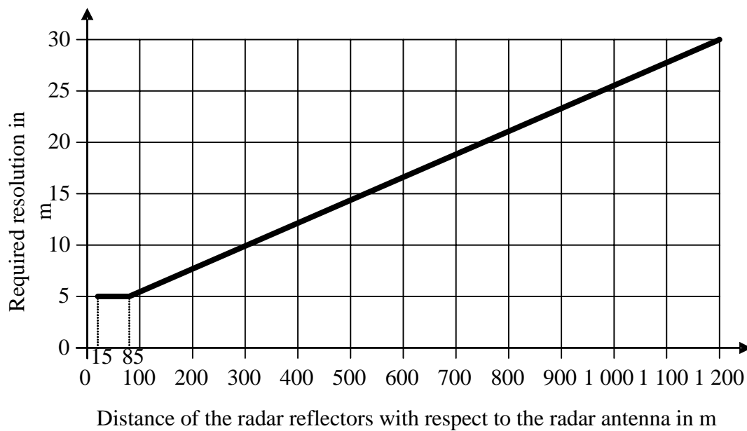
Figure B.3.2: Required azimuthal resolution depending on the range
