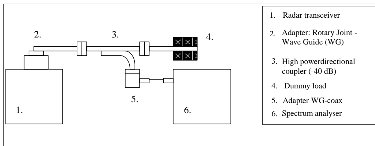
Figure C.1.1: Measurement of the operation frequency, the frequency spectrum and the pulse power
