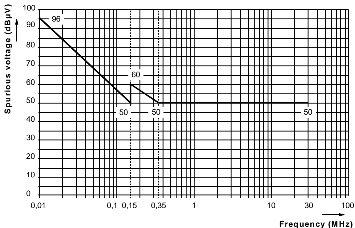
Figure 1: Conducted emissions
