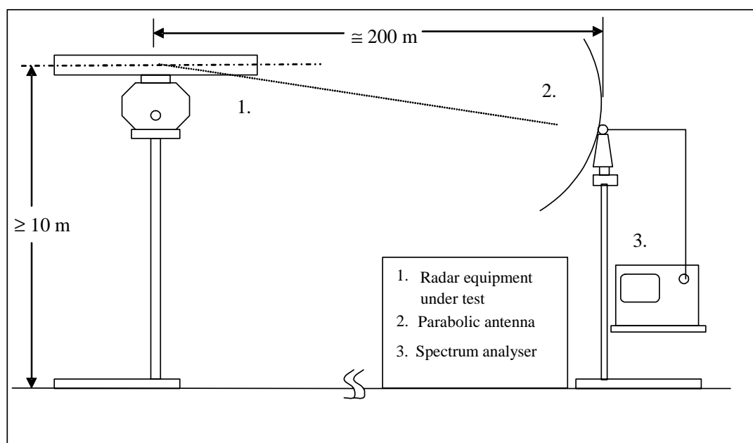
Figure C.2.1: Measurement of spurious emissions and out of band emissions, placement of components
