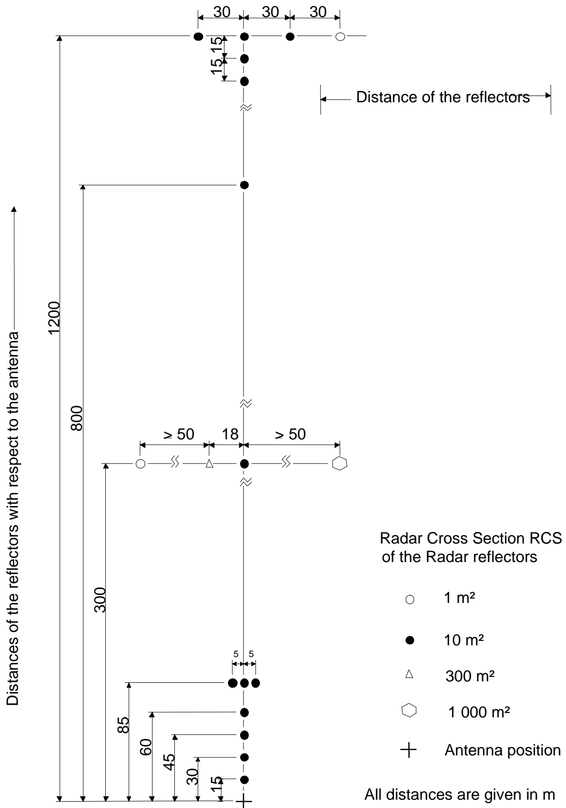
Figure A3.1: Set-up of the radar reflectors to determine the radar picture resolution
