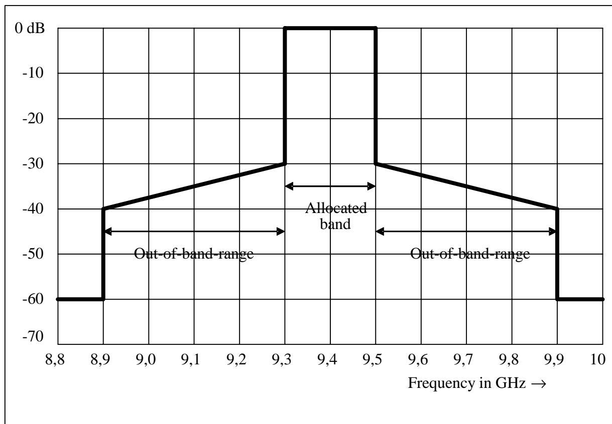
Figure C.3.1: Maximum permitted out-of-band-emissions power level
