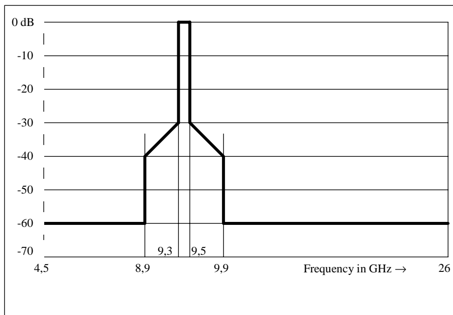
Figure C.4.1: Maximum permitted spurious emissions power level
