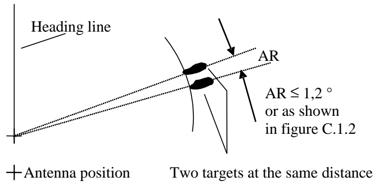
Figure B.3.1: Definition of the azimuthal resolution (AR)
