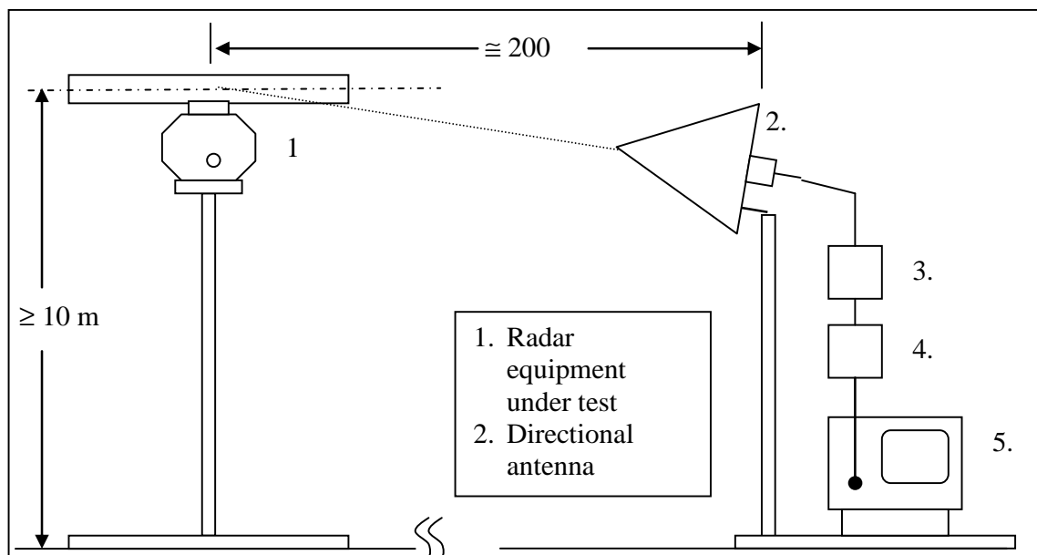
Figure D.2: Measurement of spurious emissions and out of band emissions, placement of components
