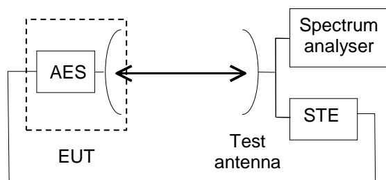
Figure 14: Test arrangement for measurement of on-axis EIRP as a function of altitude
