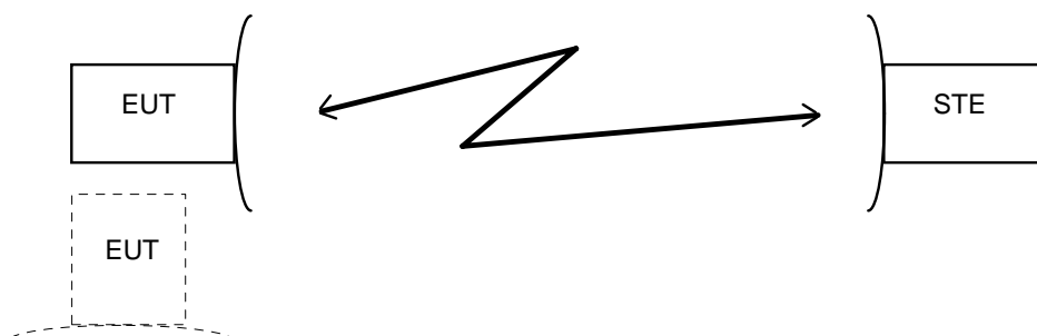
Figure 6: Test arrangement - rms pointing accuracy
