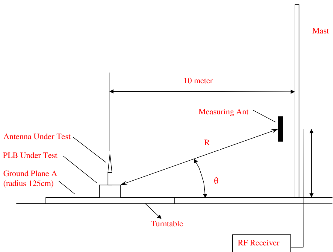
Figure A.1: Equipment Test Set-Up for Radiation Tests
