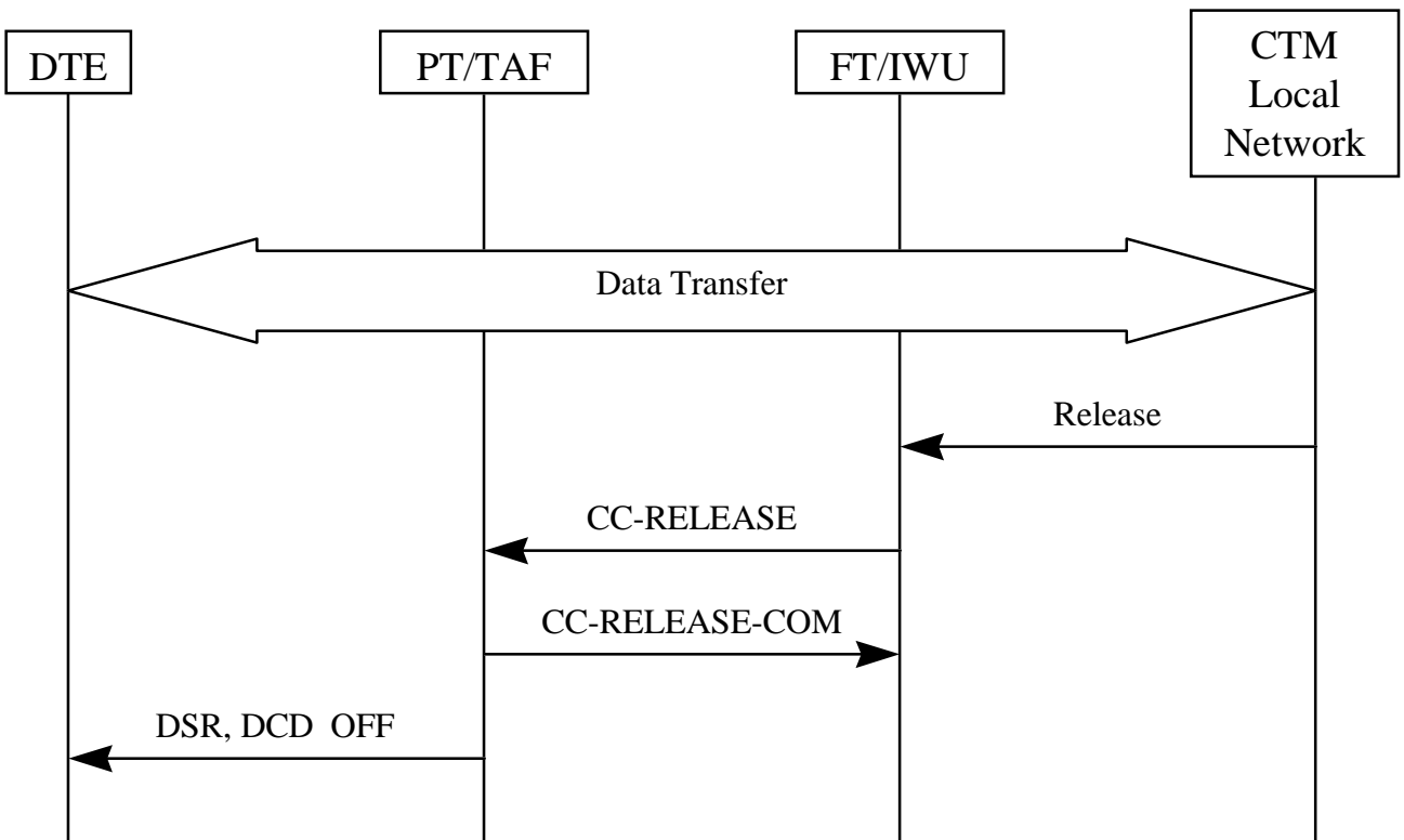
Figure B.7: Release FT initiated
