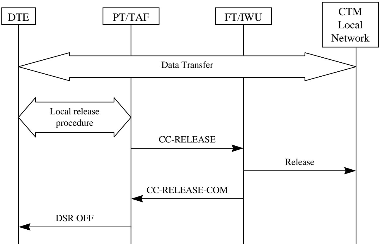
Figure B.6: Release PT initiated
