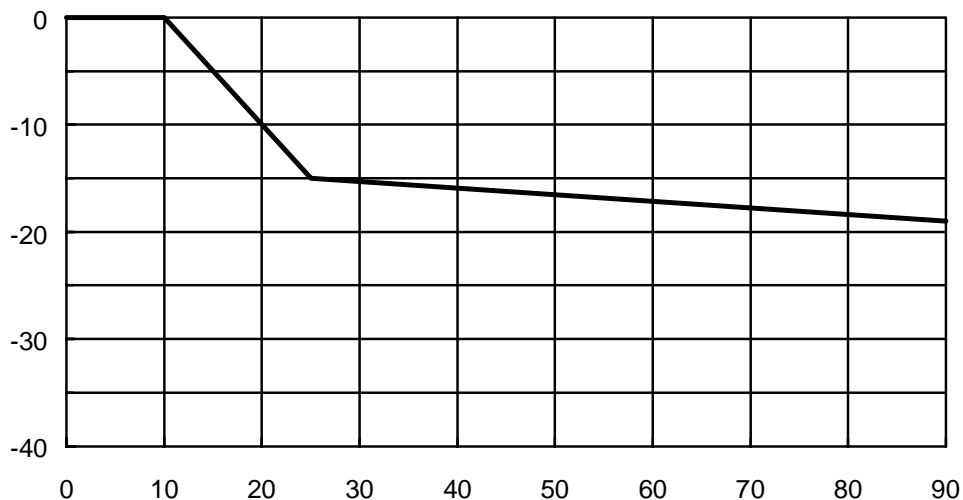
Figure 5: Symmetric CS Antenna Elevation Pattern
