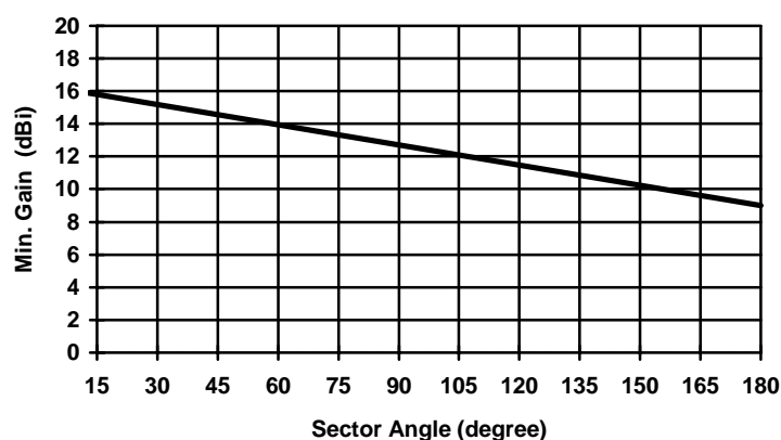
Figure 4: CS Sector Antenna Boresight Min Gain
