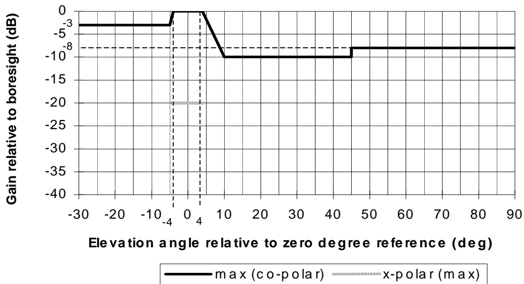
Figure 6: Asymmetric CS Antenna Elevation Patterns
