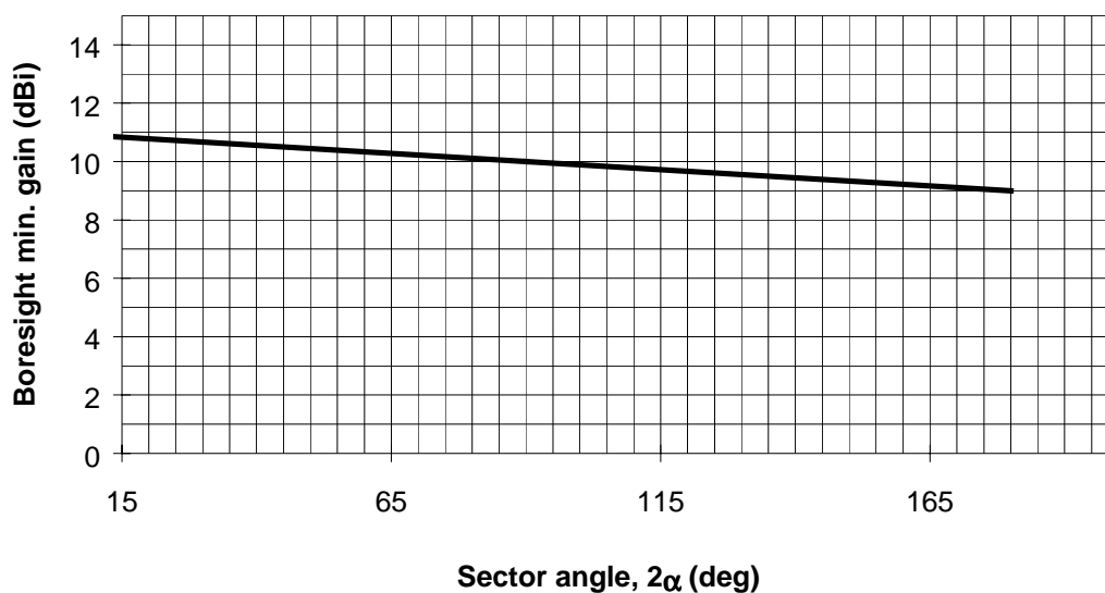
Figure 4: CS Sector Antenna Boresight Min Gain
