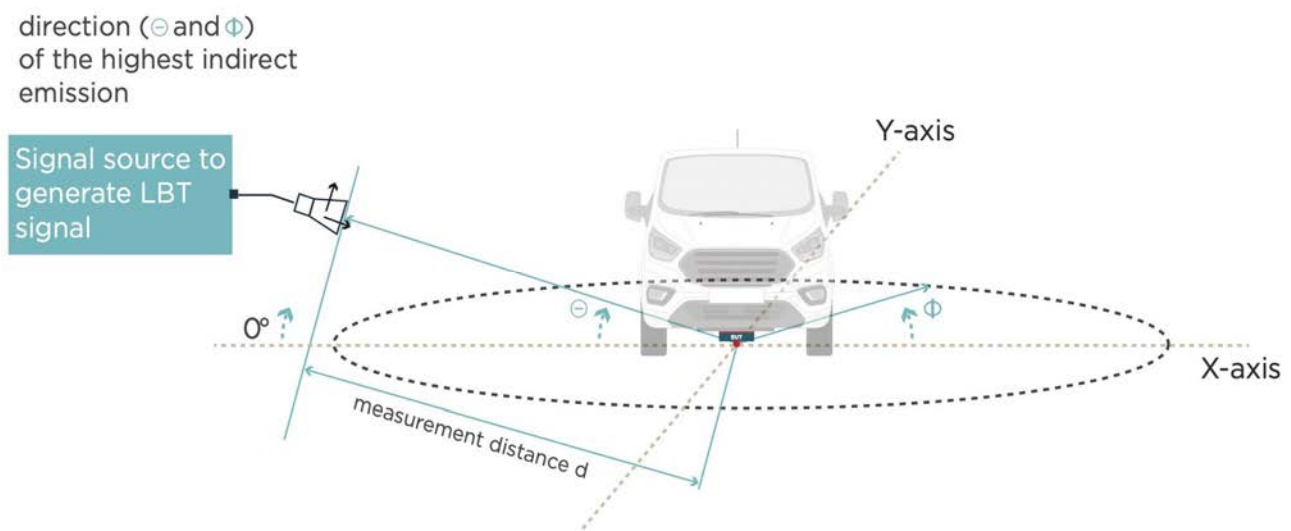
Figure 7: Set-up for LBT conformance test
