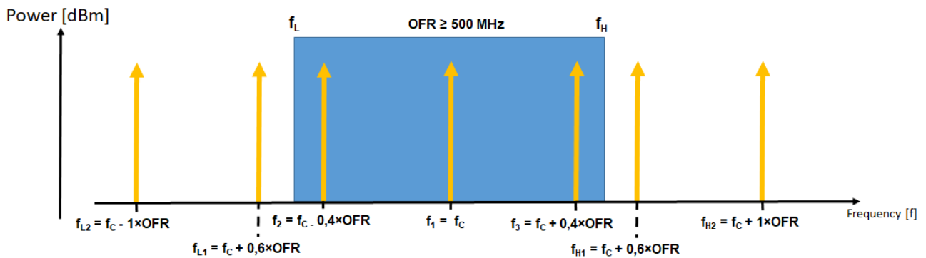
Figure D.2: Interferer test frequencies in relation to the OFR (for EUT OFR \geq 500 MHz)
