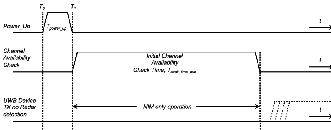
Figure 2: Example of timing for radiolocation testing of the Minimum Initial Channel Availability Check Time T_{avail\_time} , UWB DAA device intent to operate in a non NIM mode
