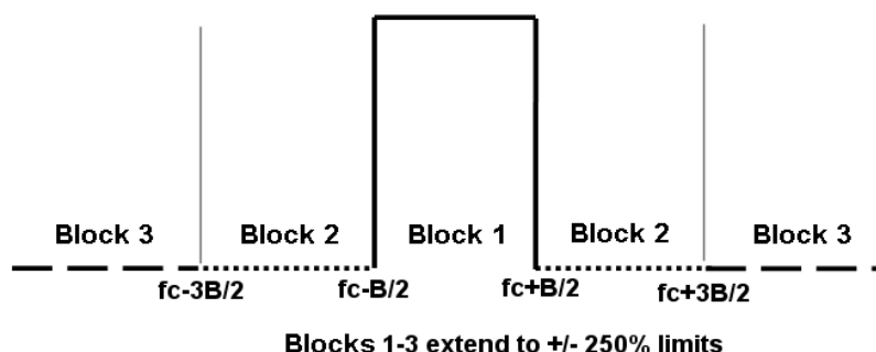
Figure 1: Measurement Mask normalized to channel bandwidth
