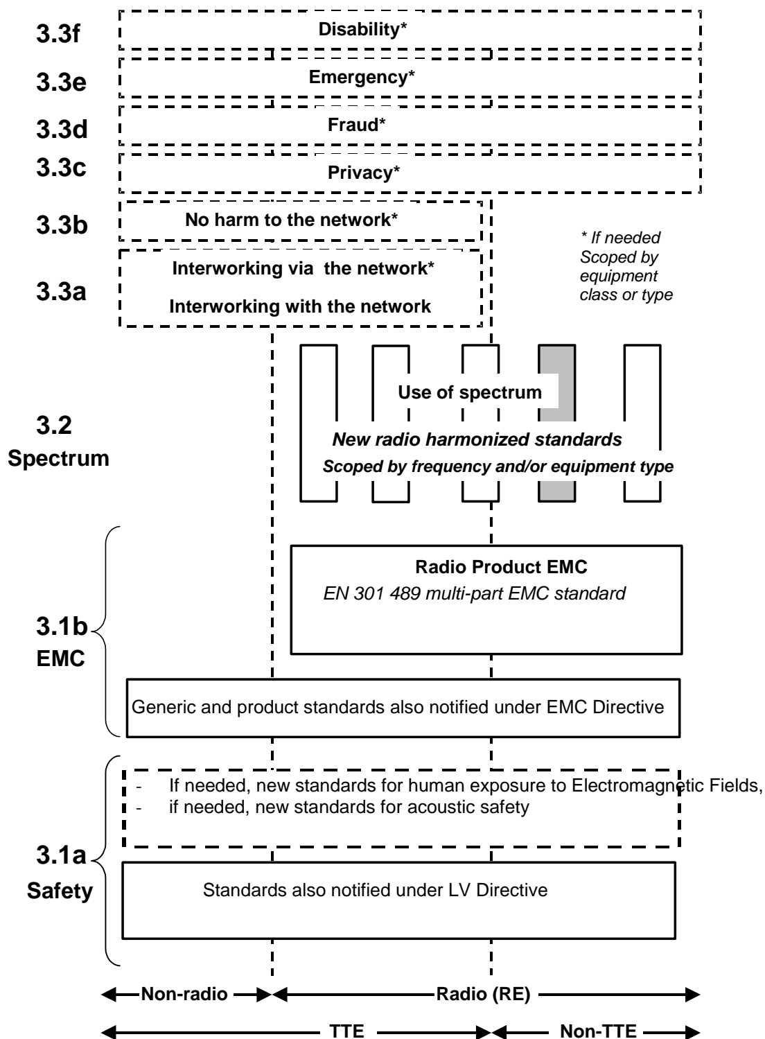
Figure 1: Modular structure for the various standards used under the R&TTE Directive [1]
