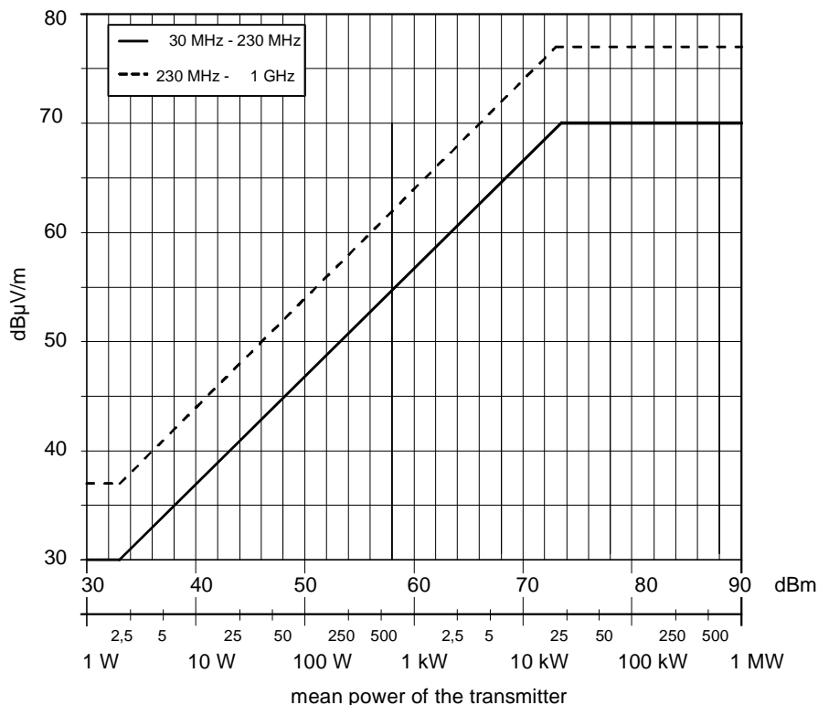
Figure 4: Enclosure port limits for FM sound broadcasting transmitters
