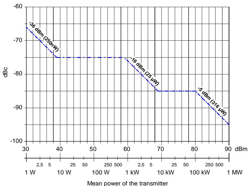
Figure 2: Spurious Emission limits for FM sound broadcasting transmitters
