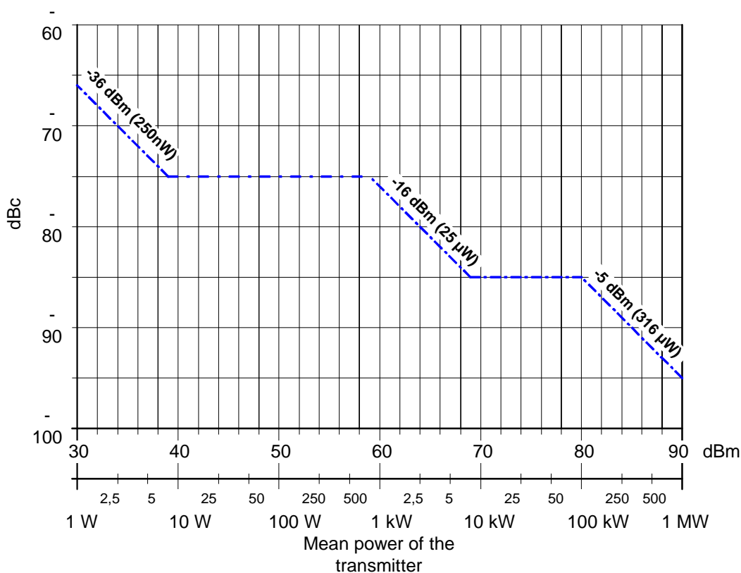
Figure 1: Spurious Emission limits for FM sound broadcasting transmitters
