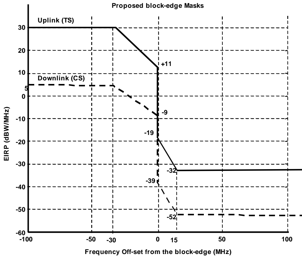
Figure A.1: Tx EIRP spectral density block mask from ECC Recommendation 01-04
