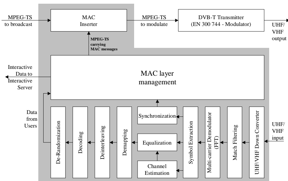
Figure 6: Conceptual Block Diagram for the Base Station
