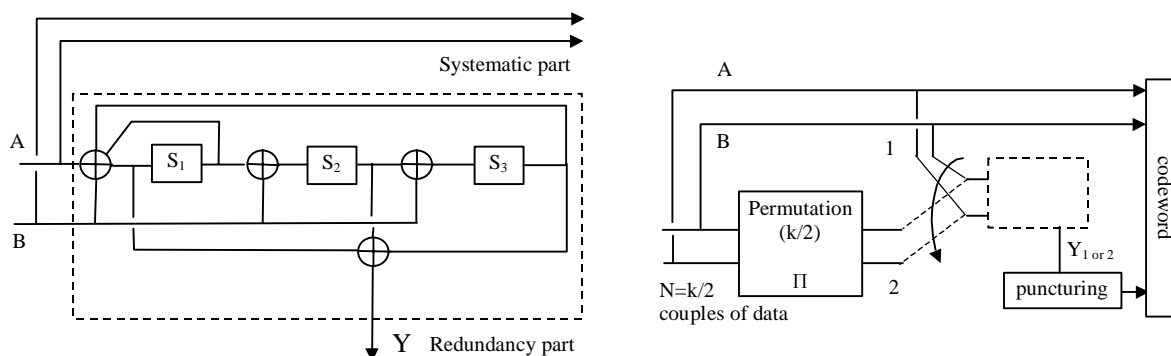
Figure 15: Encoder block diagram (turbo code)
