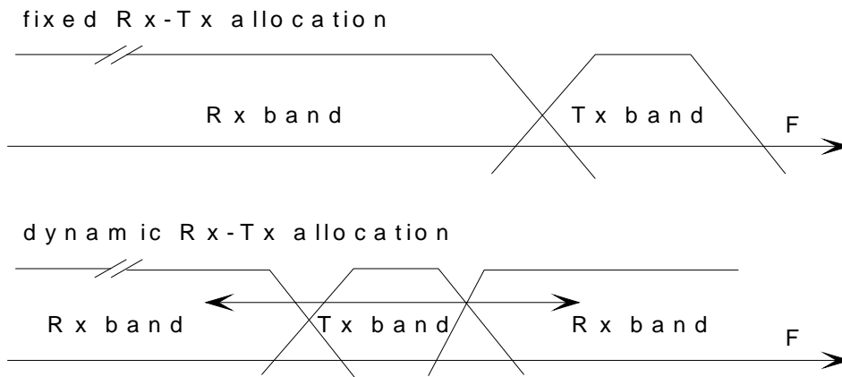
Figure 55: Possible Frequency Allocation Techniques
