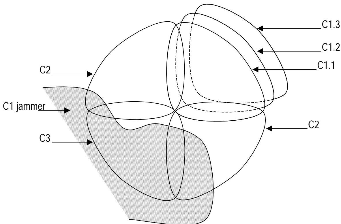
Figure 43: Sectoring a DVB-T cell; frequency re-use; minimizing interference; several US channels inside one sector
