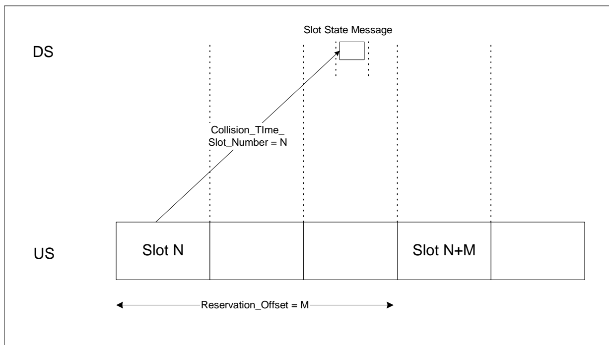
Figure 47: Examples of configurable Slot_State message delay
