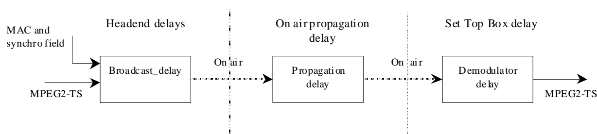
Figure 11: System Model for Timing Analysis
