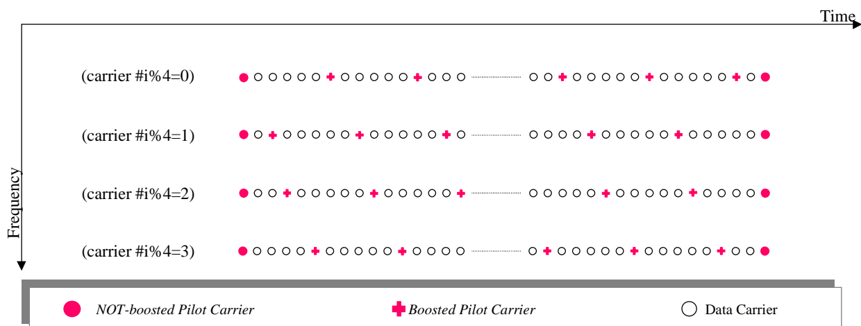
Figure 27: Pilot insertion scheme for the BS2 mini-bursts
