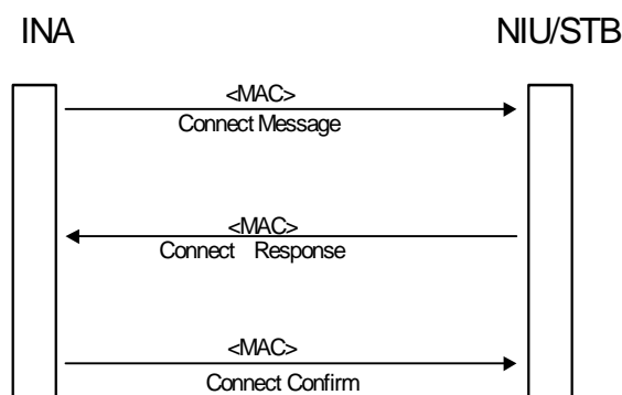
Figure 48: Connection Signalling for the Initial Connection
