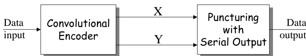
Figure 16: Convolutional encoder Block diagram
