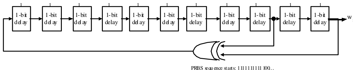
Figure 20: PRBS sequence generator for Pilot modulation
