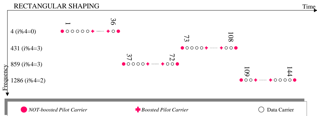
Figure 25: BS1 with frequency hopping and rectangular shaping
