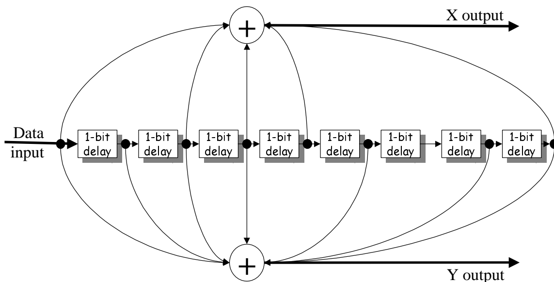
Figure 17: Convolutional Encoder Block diagram
