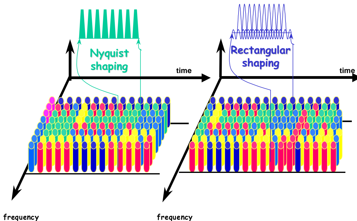
Figure 7: Illustration of the DVB-RCT Radio Frequency channel organization
