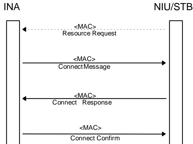
Figure 51: Connection signalling for additional connections
