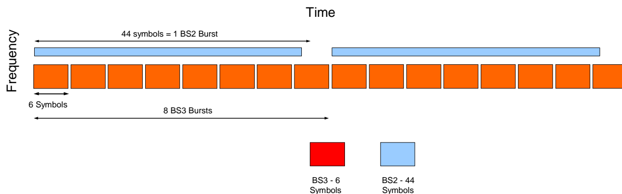
Figure 30: Transmission frame organization for MAS3
