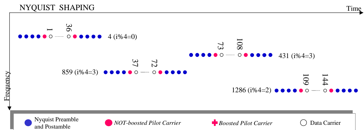
Figure 26: BS1 with frequency hopping and Nyquist shaping
