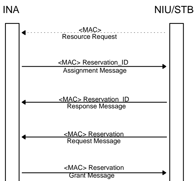
Figure 53: Reservation access signalling
