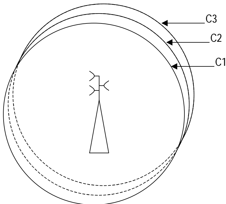
Figure 42: Several US channels in a DVB-T cell
