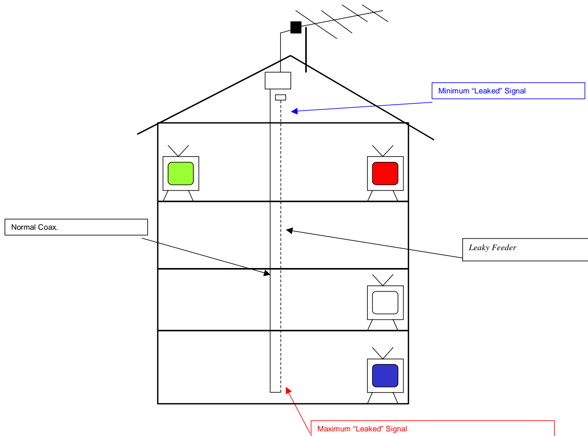
Figure 62: Multiple Dwelling Units (MDU) antenna arrangements
