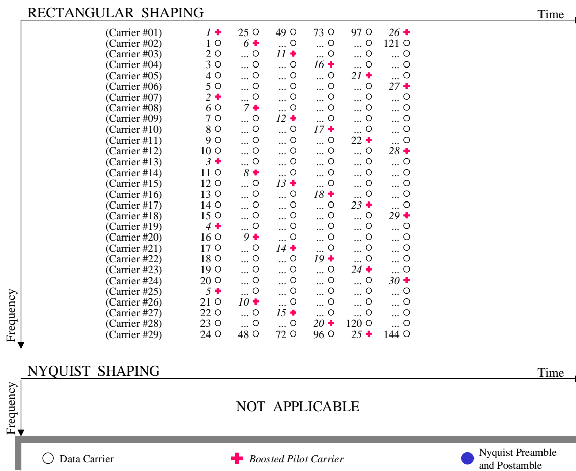
Figure 29: Illustration of BS3 structure
