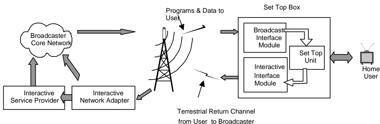
Figure 4: Illustration of the DVB-RCT network
