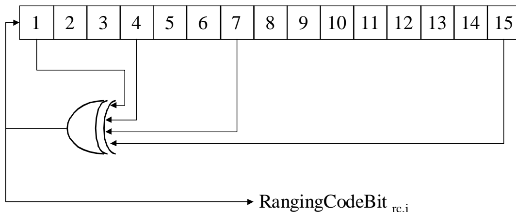
Figure 21: PRBS generator for Ranging Codes
