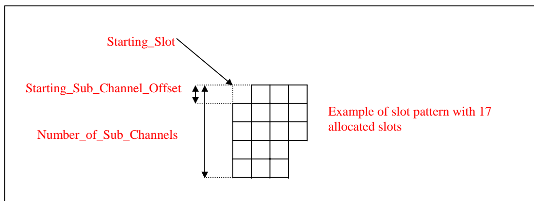
Figure 49: Slot Pattern Structure
