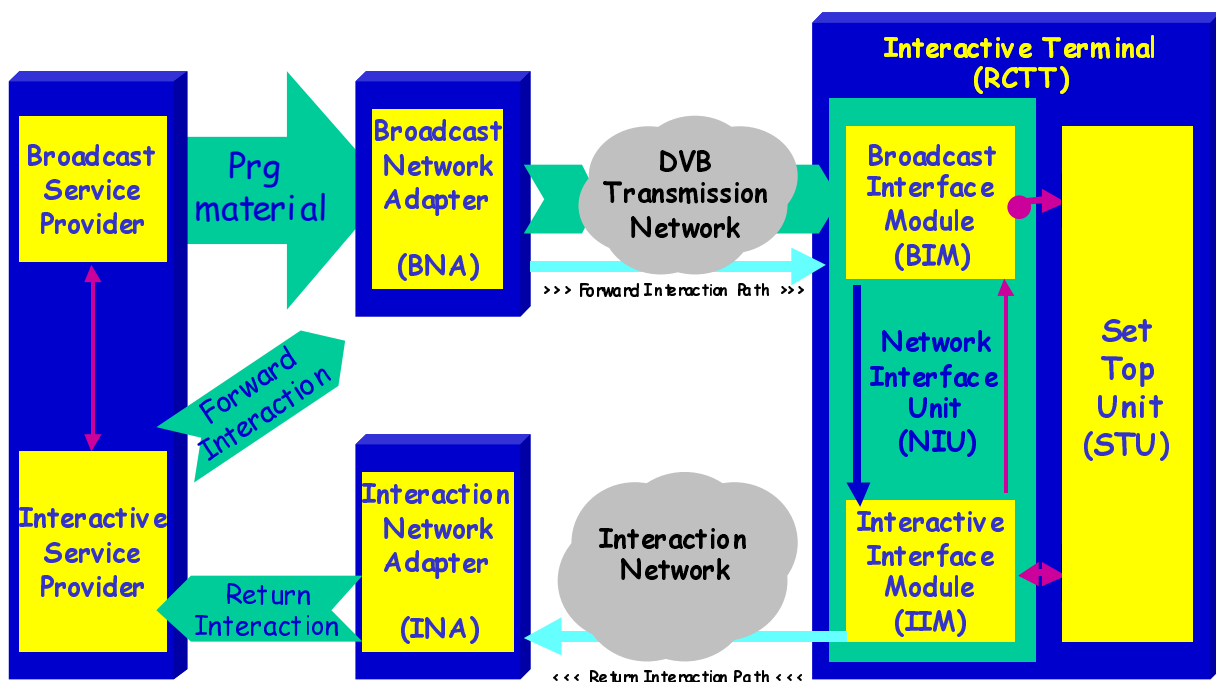
Figure 3: Reference Model for Terrestrial Interactive Systems
