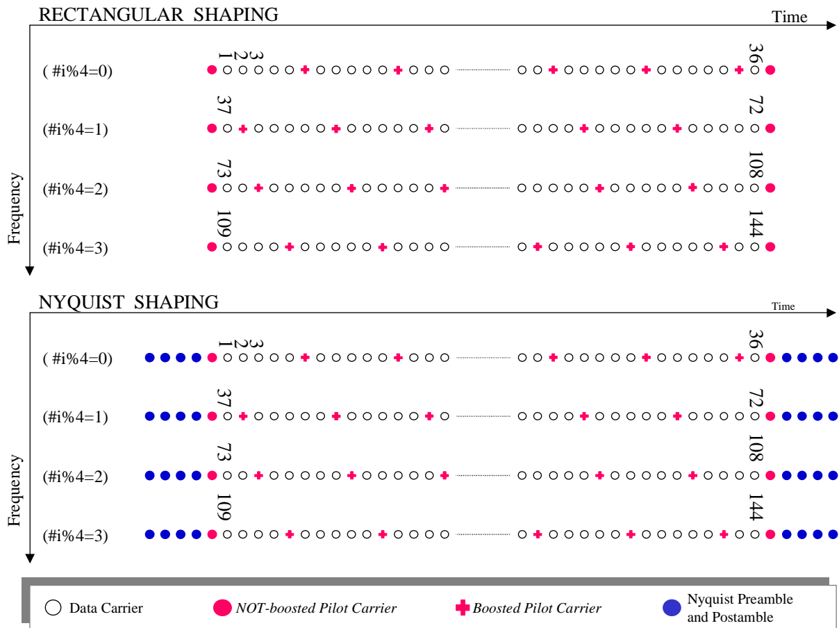
Figure 28: BS2 with Rectangular and Nyquist shaping
