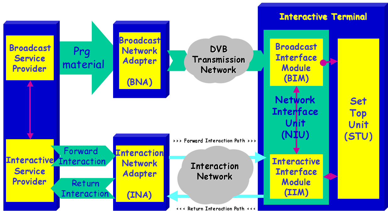
Figure 2: A generic system Reference Model for Interactive Systems
