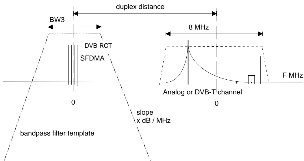
Figure 59: Definition of Duplex Distance
