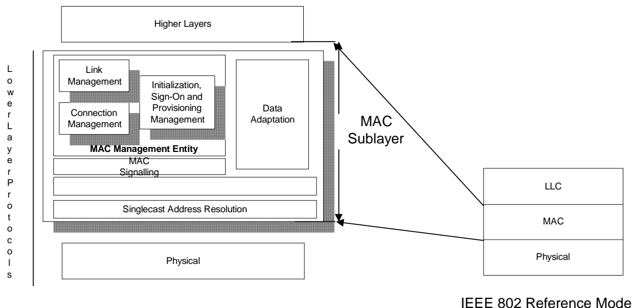
Figure 39: MAC Reference Model
