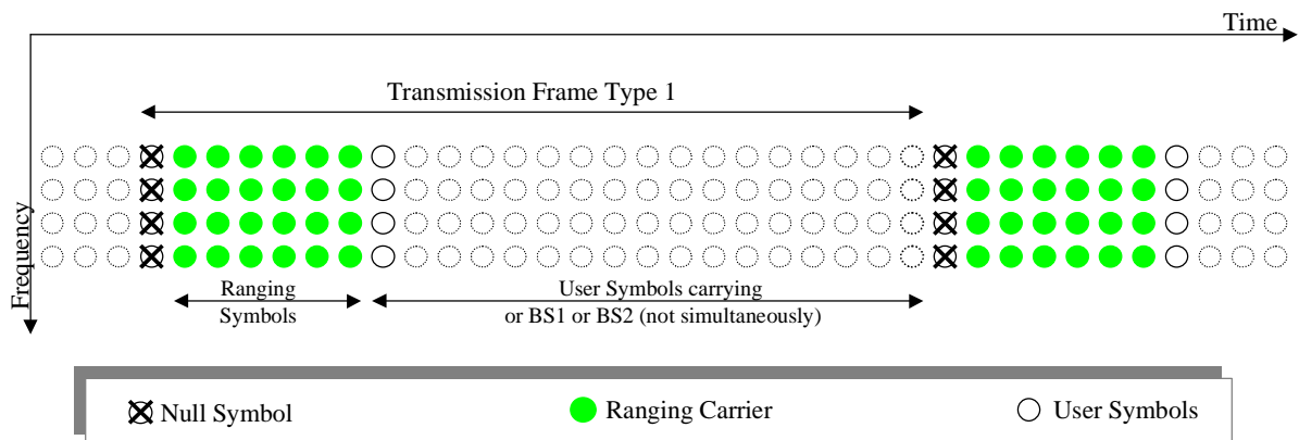
Figure 9: Organization of the TF1 frame (time domain)
