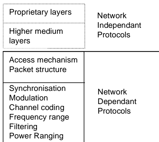
Figure 1: Layer structure for generic system reference model
