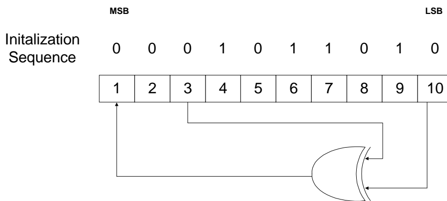
Figure 18: PRBS generator for random interleaving
