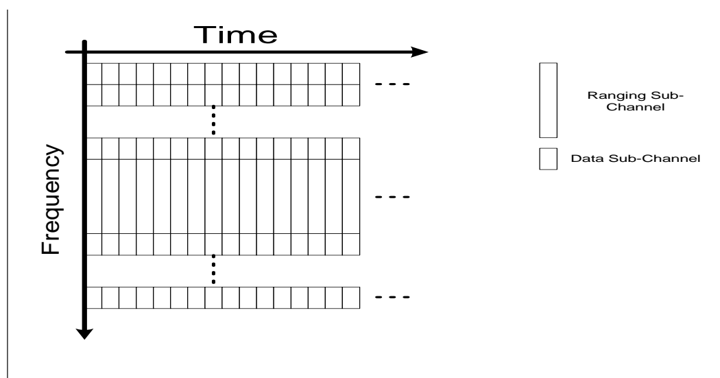
Figure 40: Example of frequency over time logical channels structure (TF2 case)
