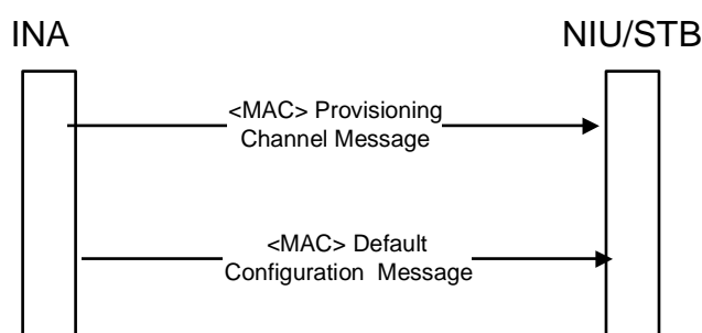
Figure 44: Initialization and Provisioning signalling
