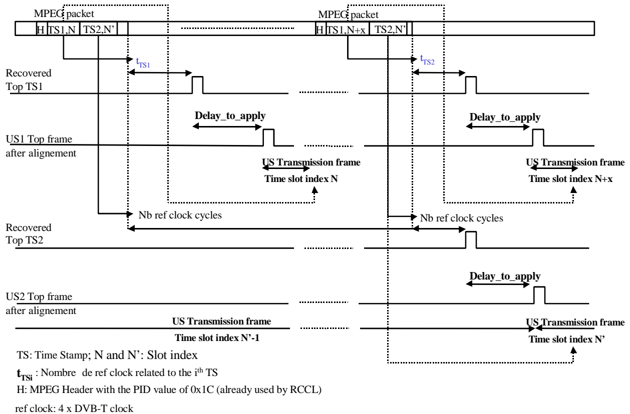
Figure 12: Time Stamp principle
