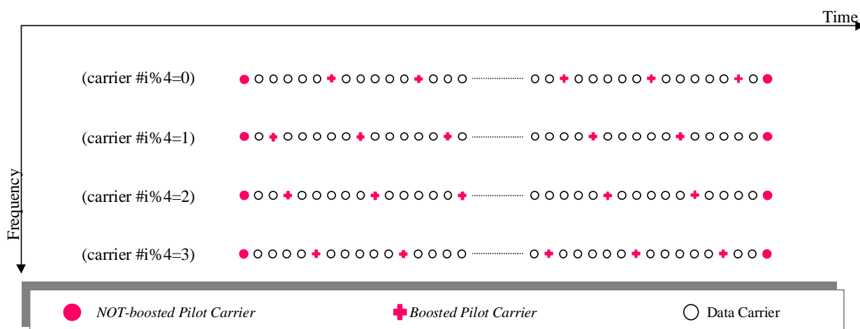
Figure 22: Pilot insertion scheme for the BS1 mini-bursts
