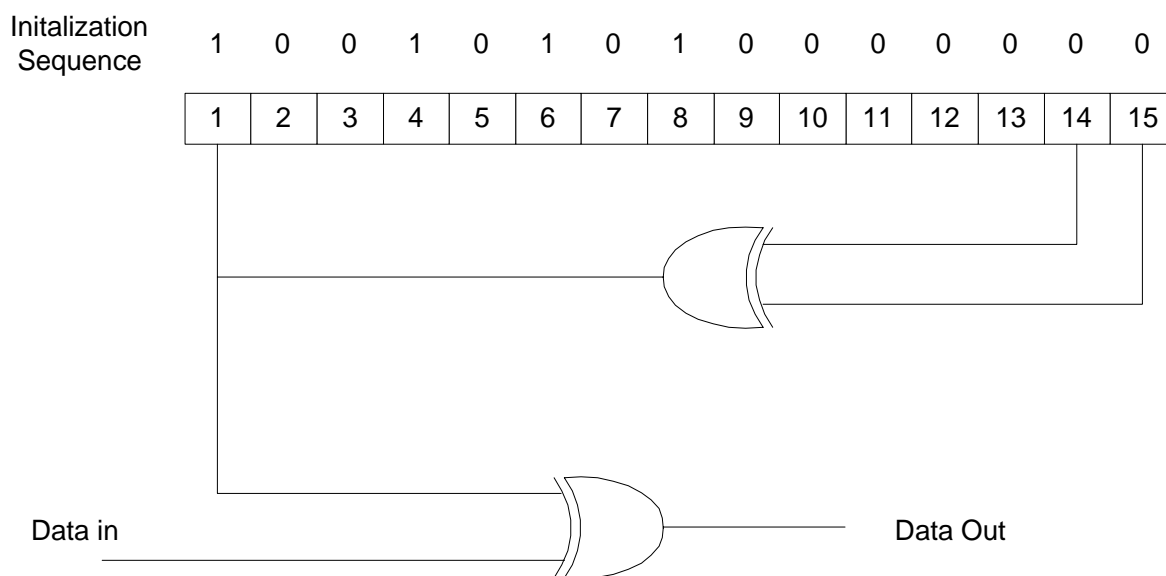
Figure 14: Block diagram for Data Randomization
