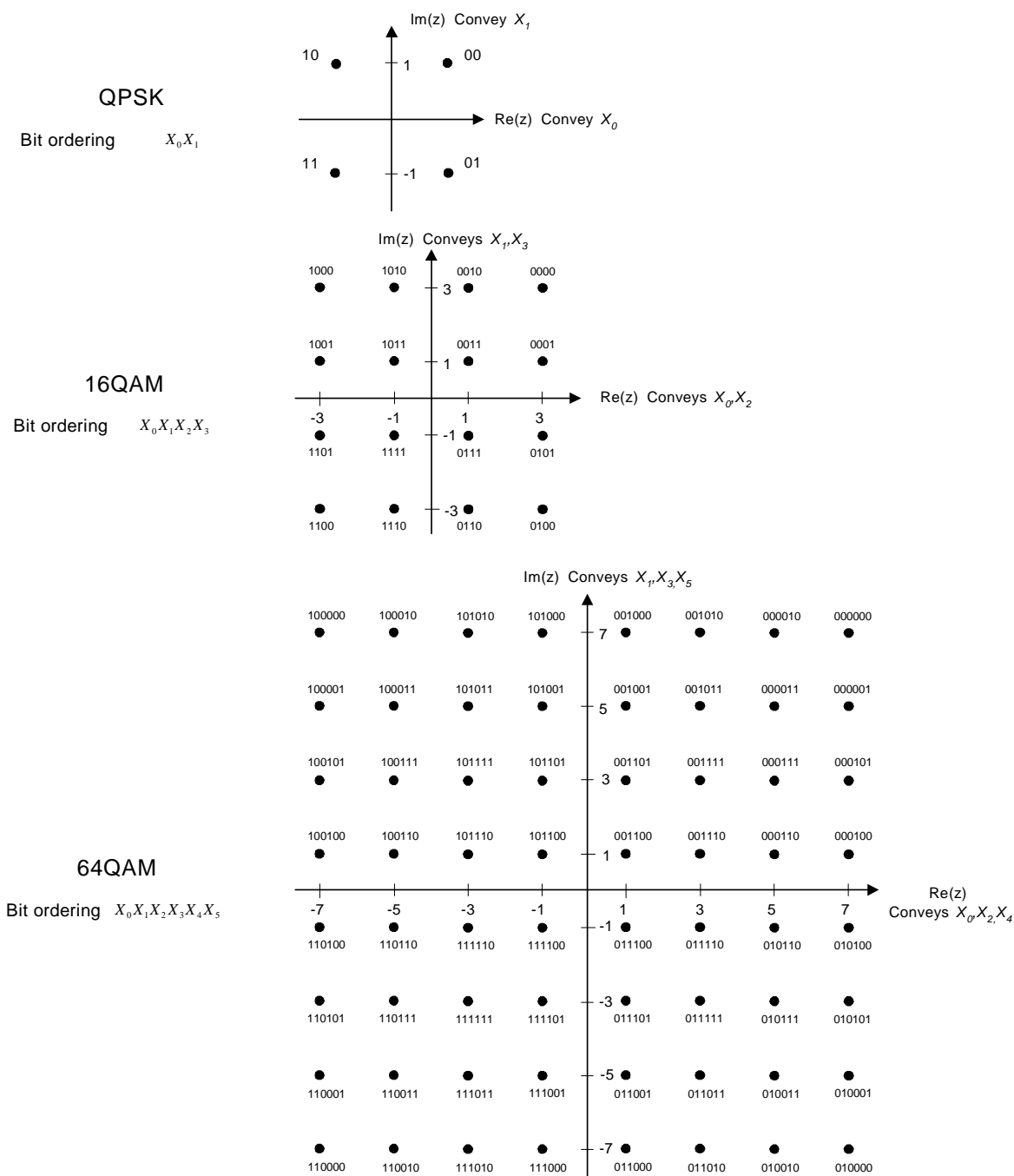
Figure 19: QPSK, 16QAM and 64QAM Constellations
