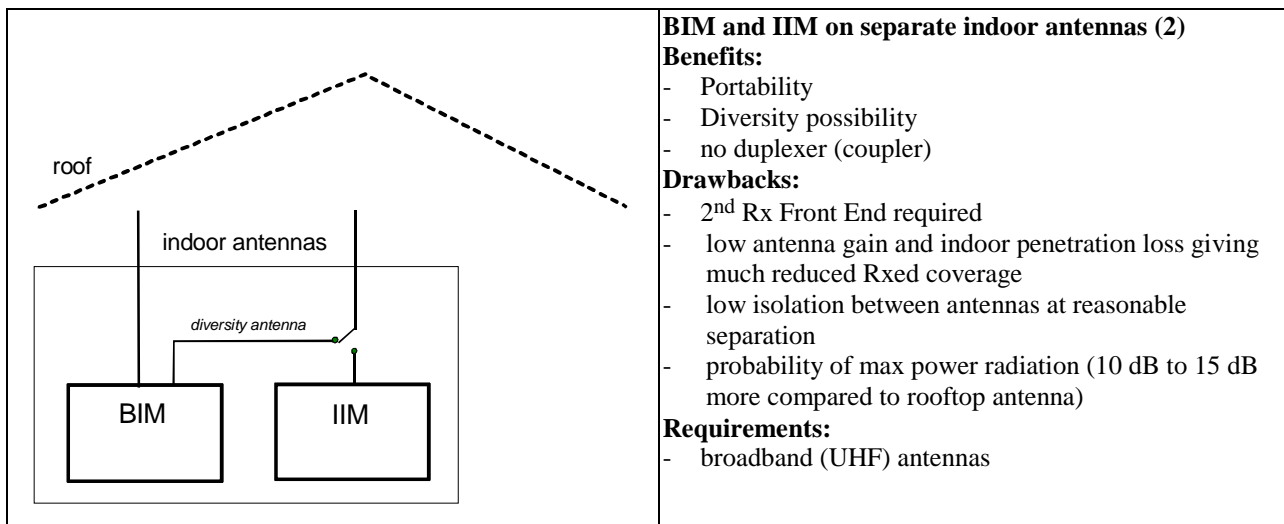
Figure 61: antenna arrangements
