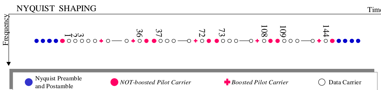
Figure 24: BS1 with Nyquist shaping and without frequency hopping option
