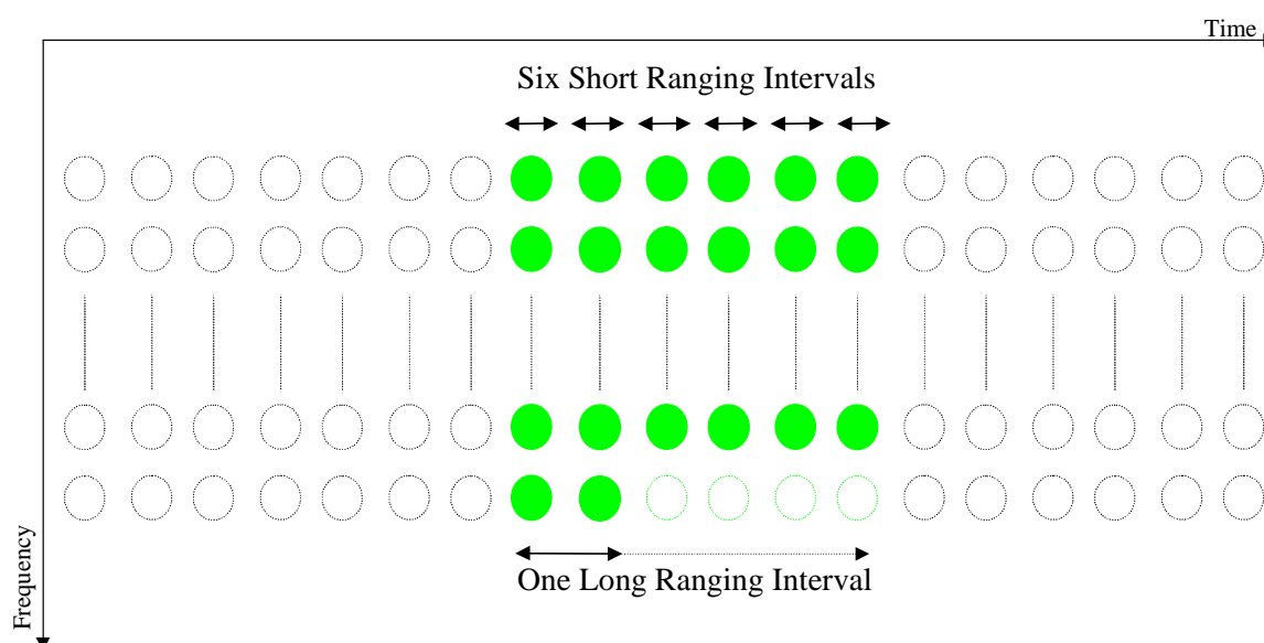
Figure 31: Basic Ranging Interval
