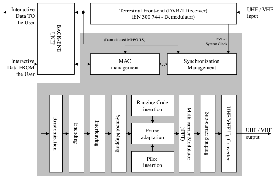
Figure 5: Conceptual Block Diagram for the DVB-RCT
