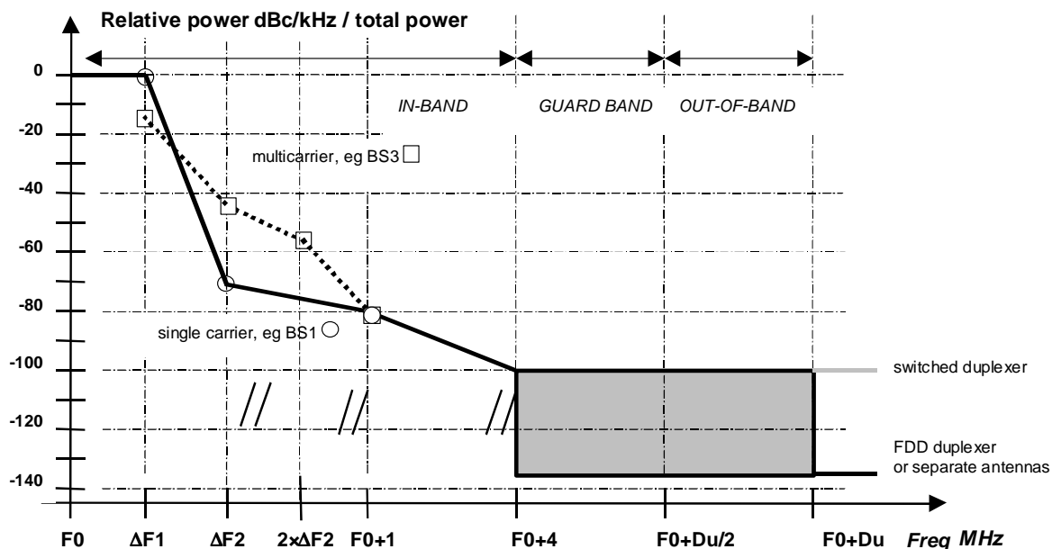
Figure 33: RF transmission power mask
