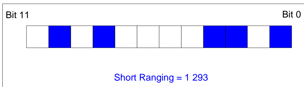
Figure 45: Example of Short/Long ranging sub-channel mapping for MAS1 or MAS2 in 2K mode
