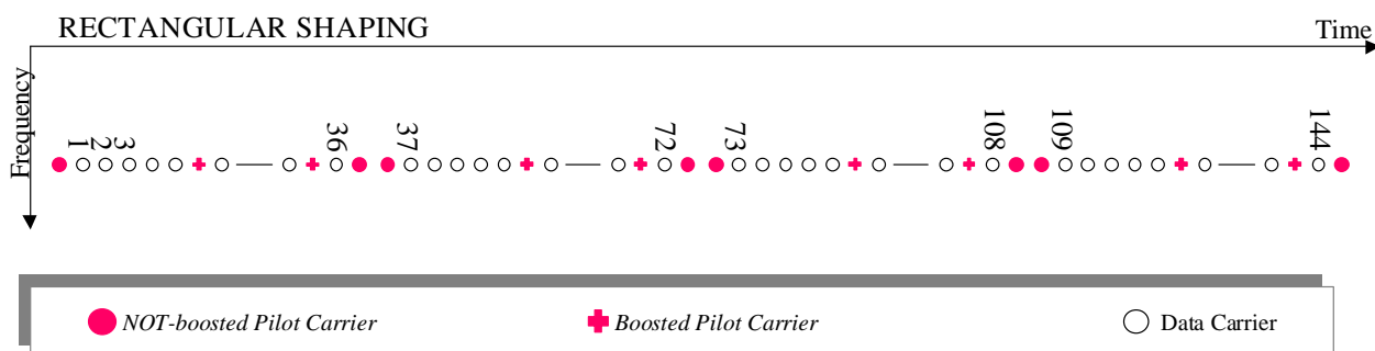
Figure 23: BS1 with rectangular shaping and without frequency hopping option
