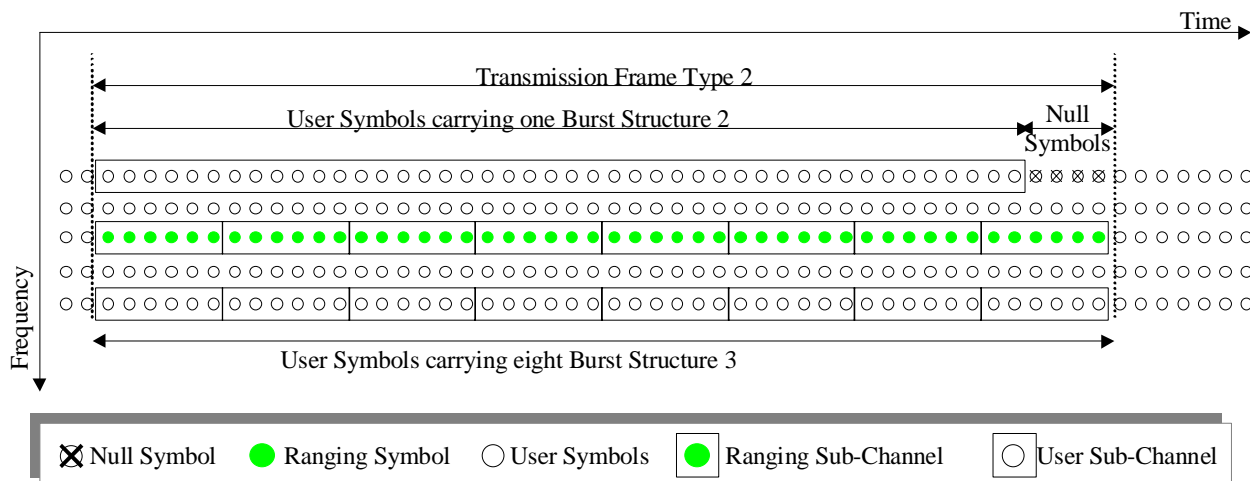
Figure 10: Organization of TF2 frame structure (time domain)
