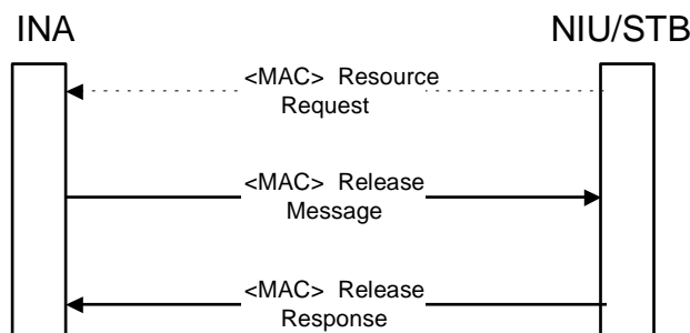
Figure 52: Connection release signalling
