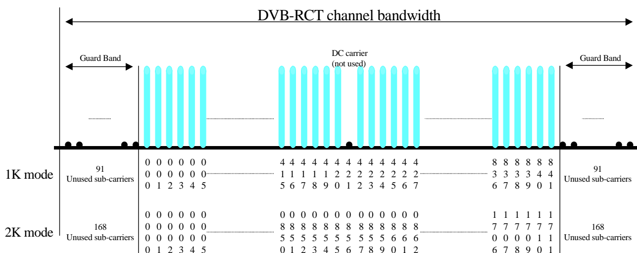
Figure 8: DVB-RCT channel organization for the 1K and 2K modes
