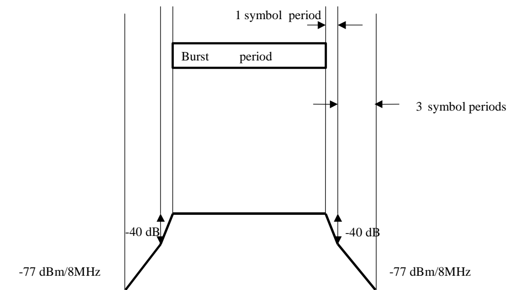
Figure 32: Switching performance of the UHF return channel modulator
