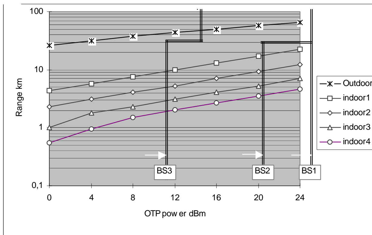
Figure 60: Service ranges/transmission power for BS1, BS2 and BS3
