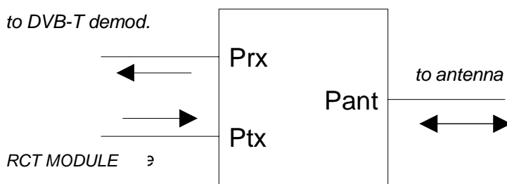
Figure 56: Duplexer device synopsis
