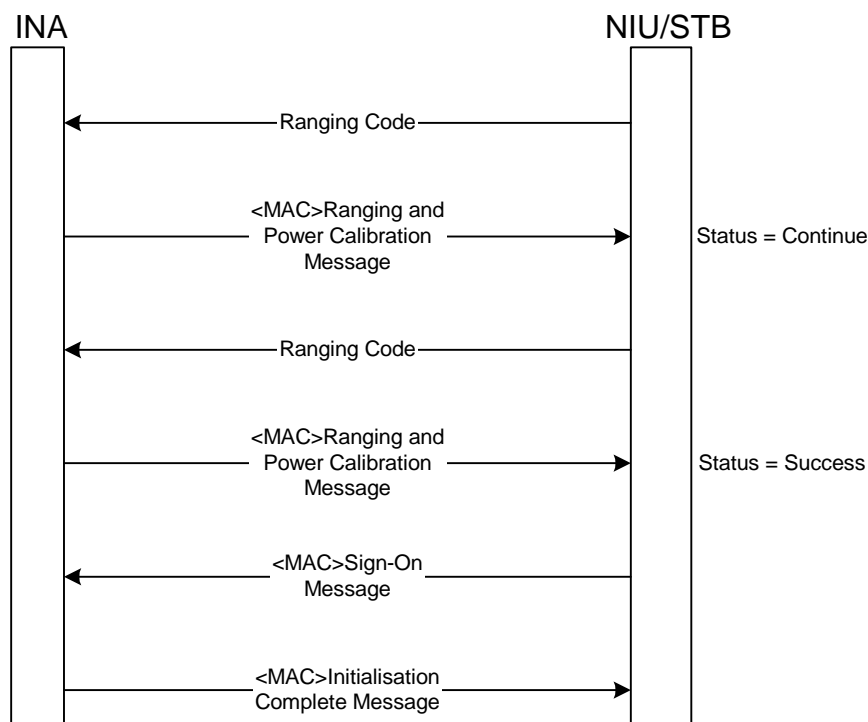
Figure 46: Ranging and Calibration Signalling
