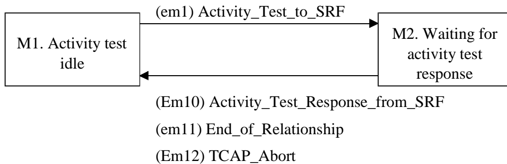
Figure 23: Activitytest FSM
