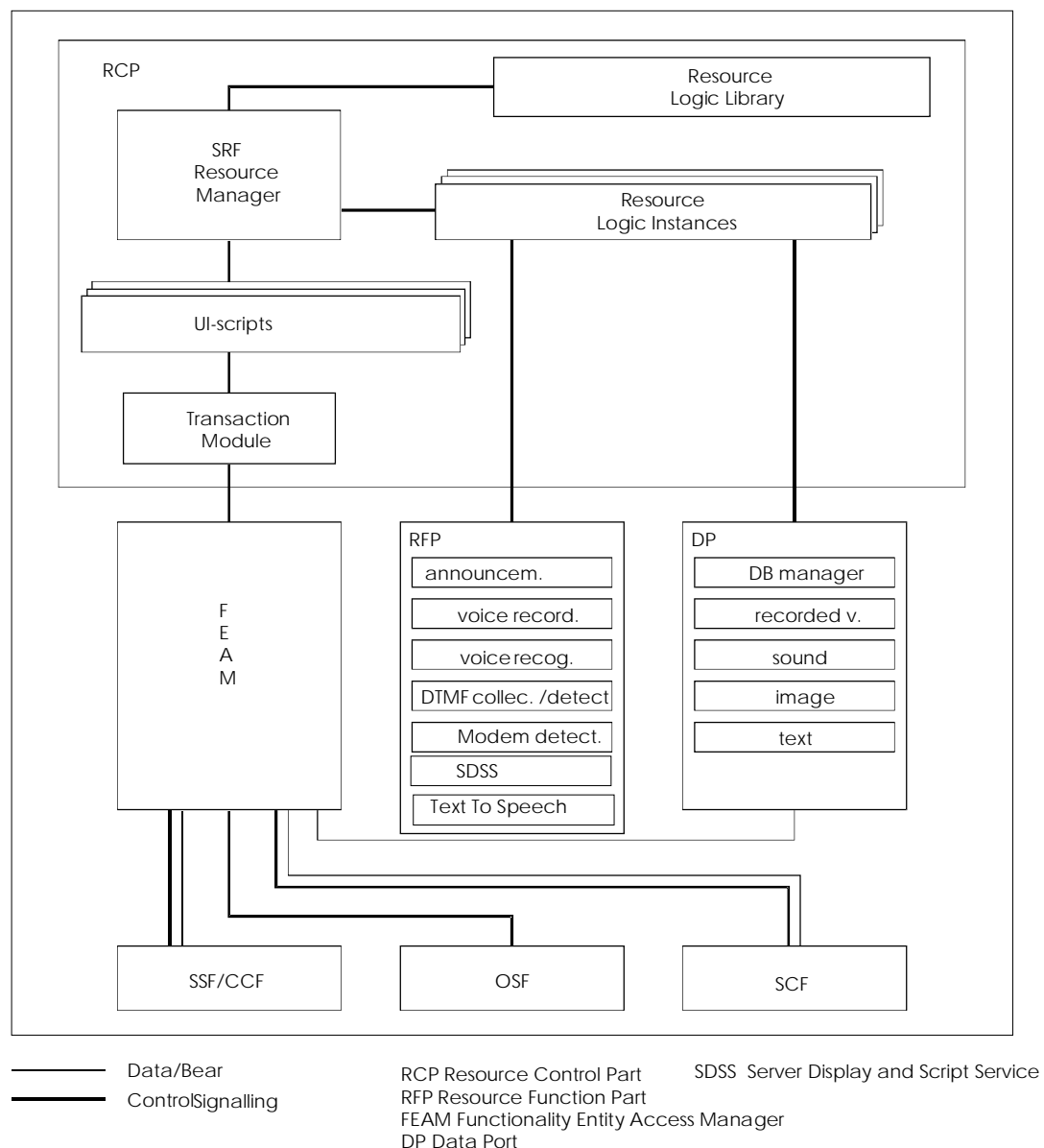
Figure 1: SRF FE Model
