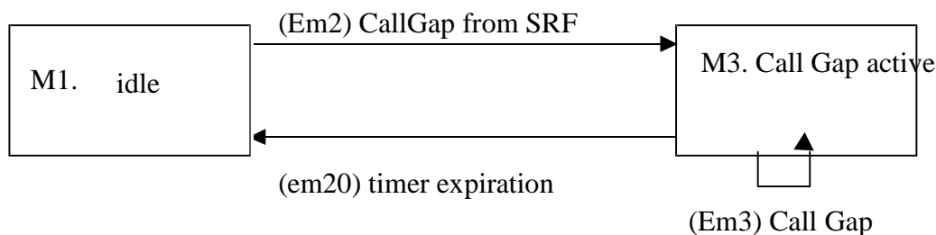
Figure 24: CallGap FSM
