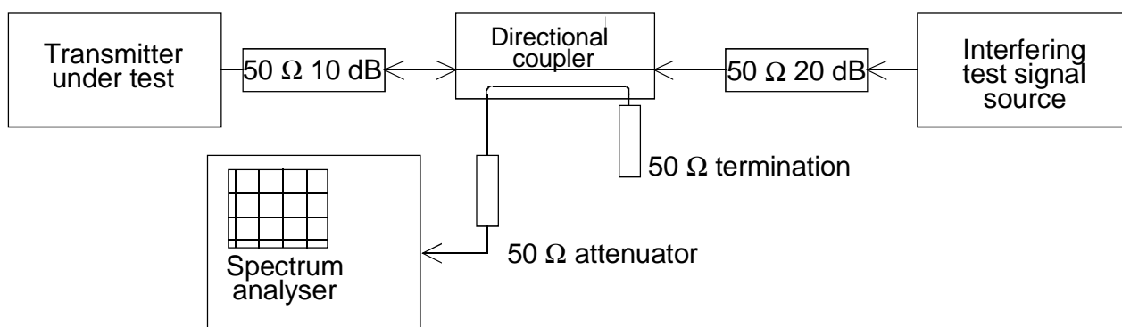
Figure 7: Measurement arrangement
