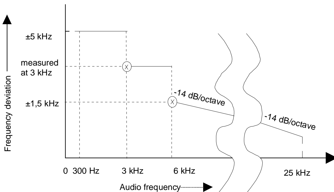
Figure 1: Frequency deviation
